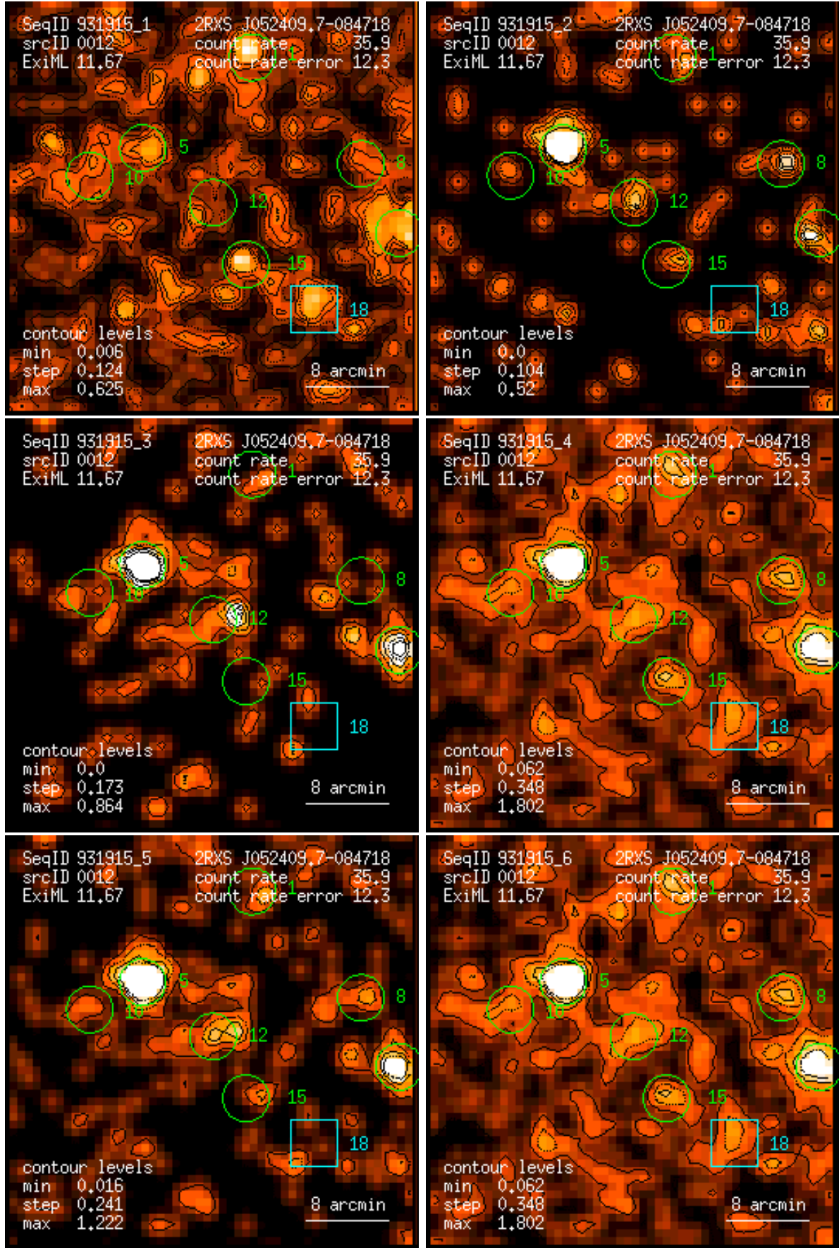
Figure 12: RASS 931915: detection 0012: band rate images, Gaussian filter: (1) PSPC channels 11 – 41, (2) 52 – 90, (3) 91 – 201, (4) 11 – 235, (5) 52 – 201, (6) 11 – 201. Broad band rates in counts/ks. Band rate contour levels in counts/ks/arcmin 2 .
