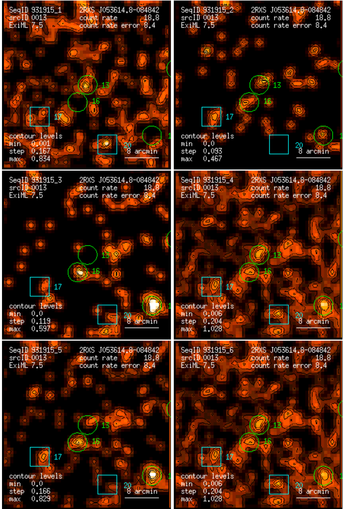
Figure 13: RASS 931915: detection 0013: band rate images, Gaussian filter: (1) PSPC channels 11 – 41, (2) 52 – 90, (3) 91 – 201, (4) 11 – 235, (5) 52 – 201, (6) 11 – 201. Broad band rates in counts/ks. Band rate contour levels in counts/ks/arcmin 2 .
