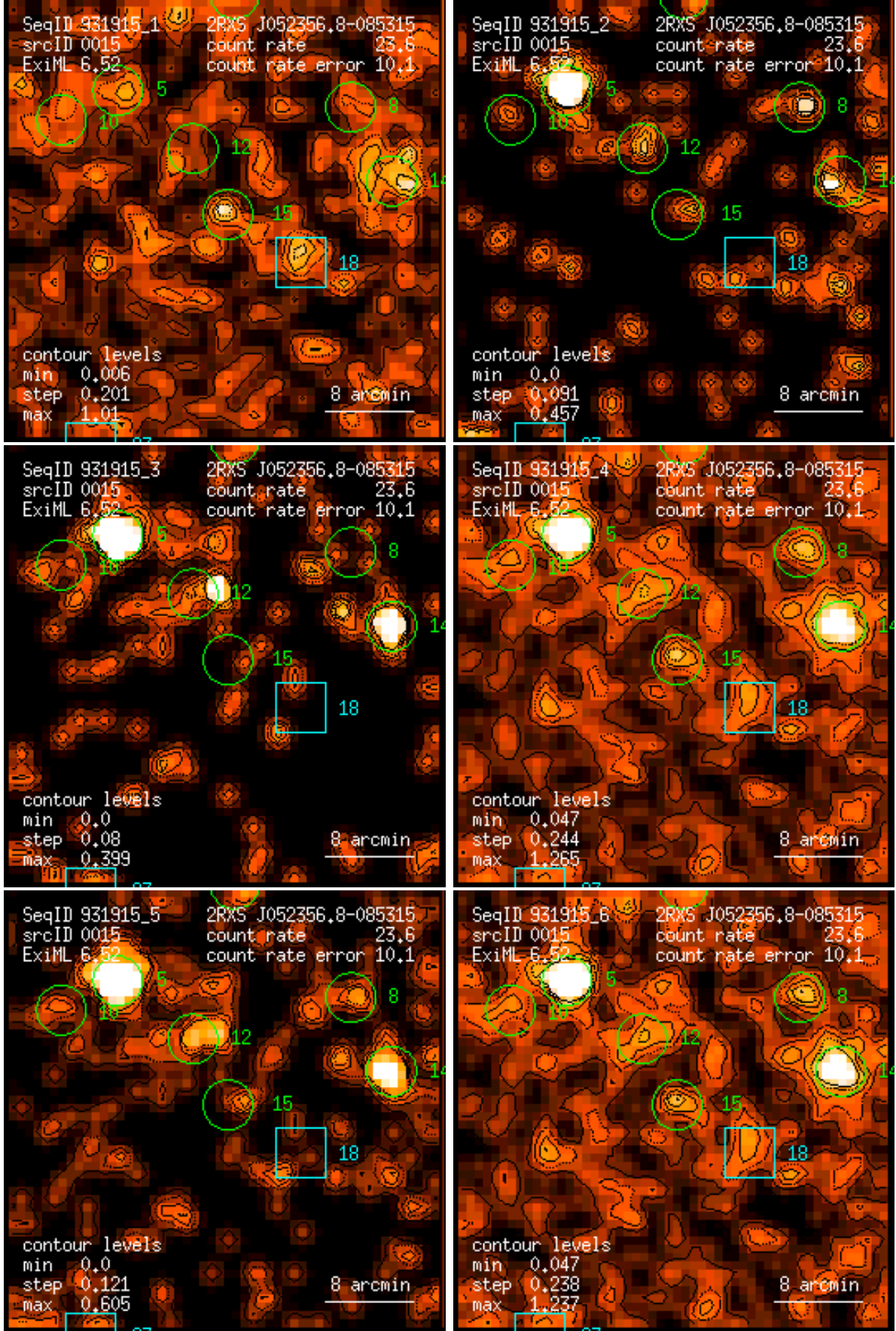
Figure 15: RASS 931915: detection 0015: band rate images, Gaussian filter: (1) PSPC channels 11 – 41, (2) 52 – 90, (3) 91 – 201, (4) 11 – 235, (5) 52 – 201, (6) 11 – 201. Broad band rates in counts/ks. Band rate contour levels in counts/ks/arcmin 2 .
