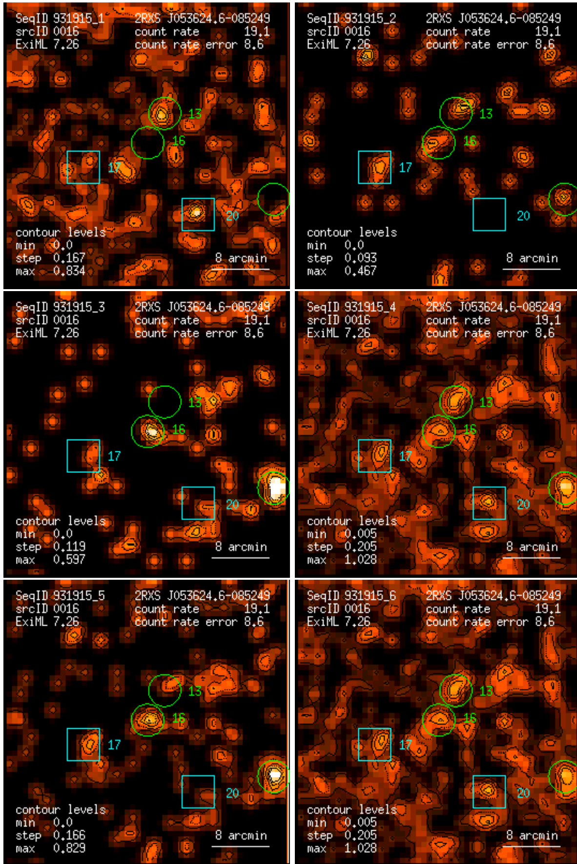
Figure 16: RASS 931915: detection 0016: band rate images, Gaussian filter: (1) PSPC channels 11 – 41, (2) 52 – 90, (3) 91 – 201, (4) 11 – 235, (5) 52 – 201, (6) 11 – 201. Broad band rates in counts/ks. Band rate contour levels in counts/ks/arcmin 2 .
