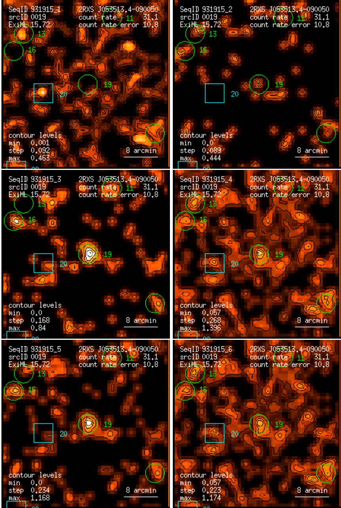
Figure 19: RASS 931915: detection 0019: band rate images, Gaussian filter: (1) PSPC channels 11 – 41, (2) 52 – 90, (3) 91 – 201, (4) 11 – 235, (5) 52 – 201, (6) 11 – 201. Broad band rates in counts/ks. Band rate contour levels in counts/ks/arcmin 2 .
