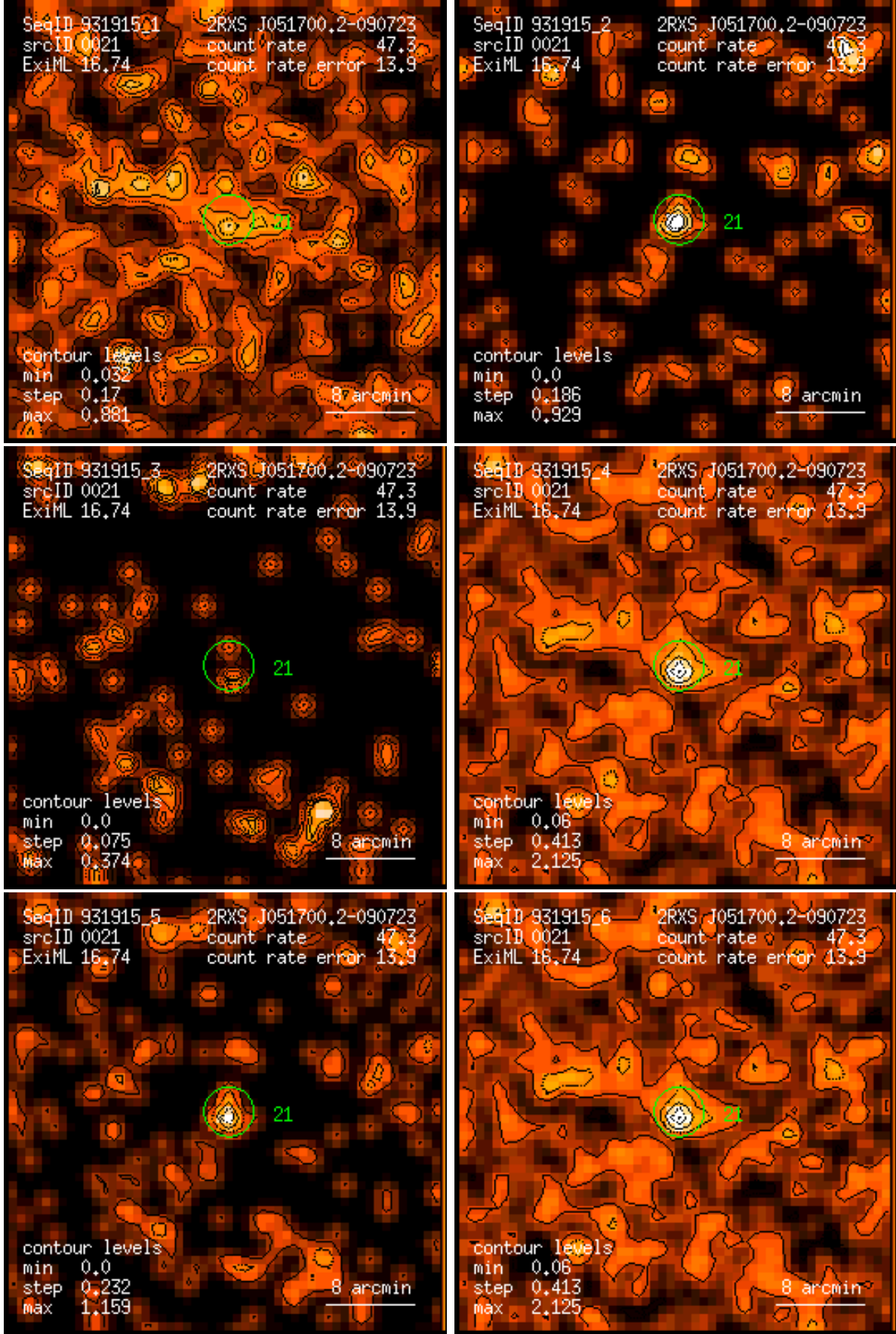
Figure 21: RASS 931915: detection 0021: band rate images, Gaussian filter: (1) PSPC channels 11 – 41, (2) 52 – 90, (3) 91 – 201, (4) 11 – 235, (5) 52 – 201, (6) 11 – 201. Broad band rates in counts/ks. Band rate contour levels in counts/ks/arcmin 2 .
