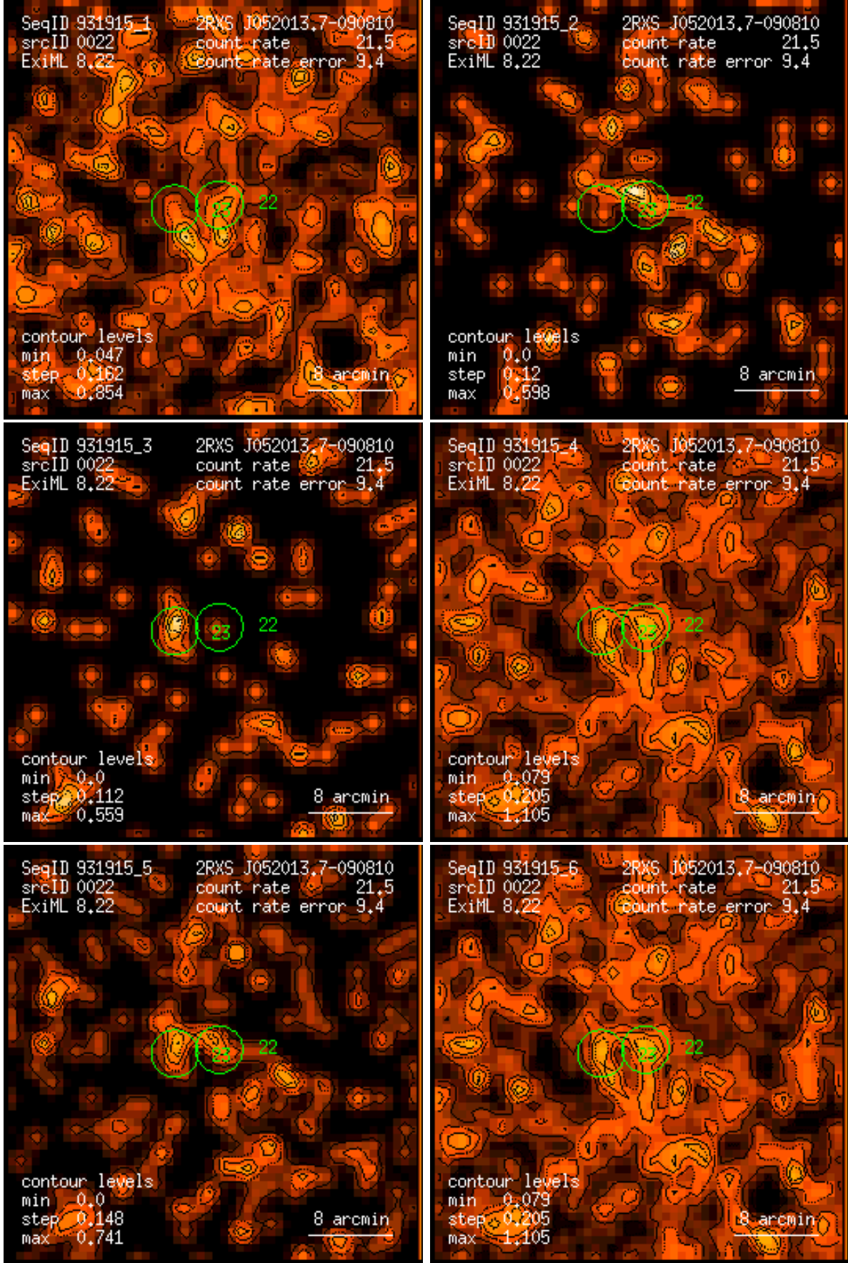
Figure 22: RASS 931915: detection 0022: band rate images, Gaussian filter: (1) PSPC channels 11 – 41, (2) 52 – 90, (3) 91 – 201, (4) 11 – 235, (5) 52 – 201, (6) 11 – 201. Broad band rates in counts/ks. Band rate contour levels in counts/ks/arcmin 2 .
