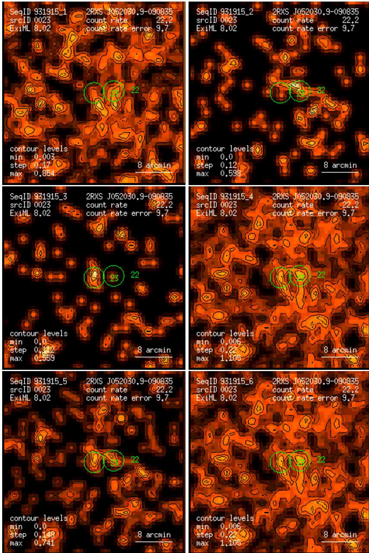
Figure 23: RASS 931915: detection 0023: band rate images, Gaussian filter: (1) PSPC channels 11 – 41, (2) 52 – 90, (3) 91 – 201, (4) 11 – 235, (5) 52 – 201, (6) 11 – 201. Broad band rates in counts/ks. Band rate contour levels in counts/ks/arcmin 2 .
