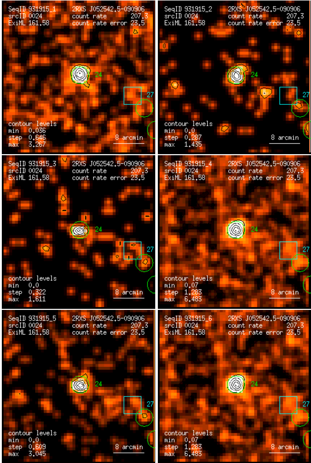
Figure 24: RASS 931915: detection 0024: band rate images, Gaussian filter: (1) PSPC channels 11 – 41, (2) 52 – 90, (3) 91 – 201, (4) 11 – 235, (5) 52 – 201, (6) 11 – 201. Broad band rates in counts/ks. Band rate contour levels in counts/ks/arcmin 2 .
