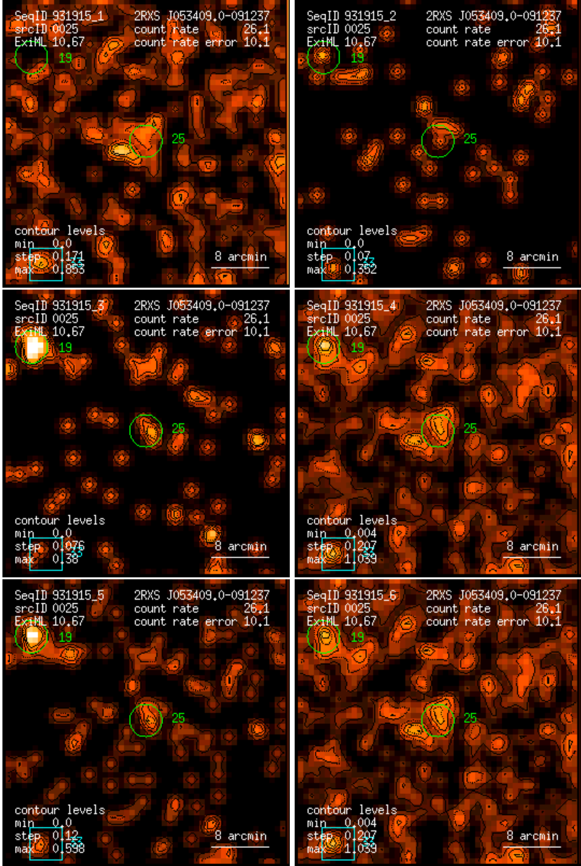
Figure 25: RASS 931915: detection 0025: band rate images, Gaussian filter: (1) PSPC channels 11 – 41, (2) 52 – 90, (3) 91 – 201, (4) 11 – 235, (5) 52 – 201, (6) 11 – 201. Broad band rates in counts/ks. Band rate contour levels in counts/ks/arcmin 2 .
