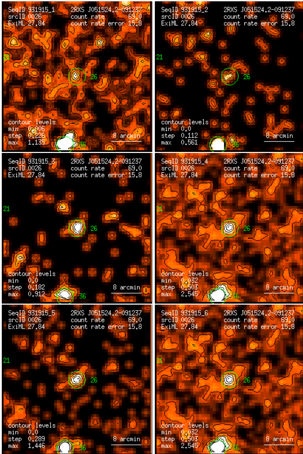
Figure 26: RASS 931915: detection 0026: band rate images, Gaussian filter: (1) PSPC channels 11 – 41, (2) 52 – 90, (3) 91 – 201, (4) 11 – 235, (5) 52 – 201, (6) 11 – 201. Broad band rates in counts/ks. Band rate contour levels in counts/ks/arcmin 2 .
