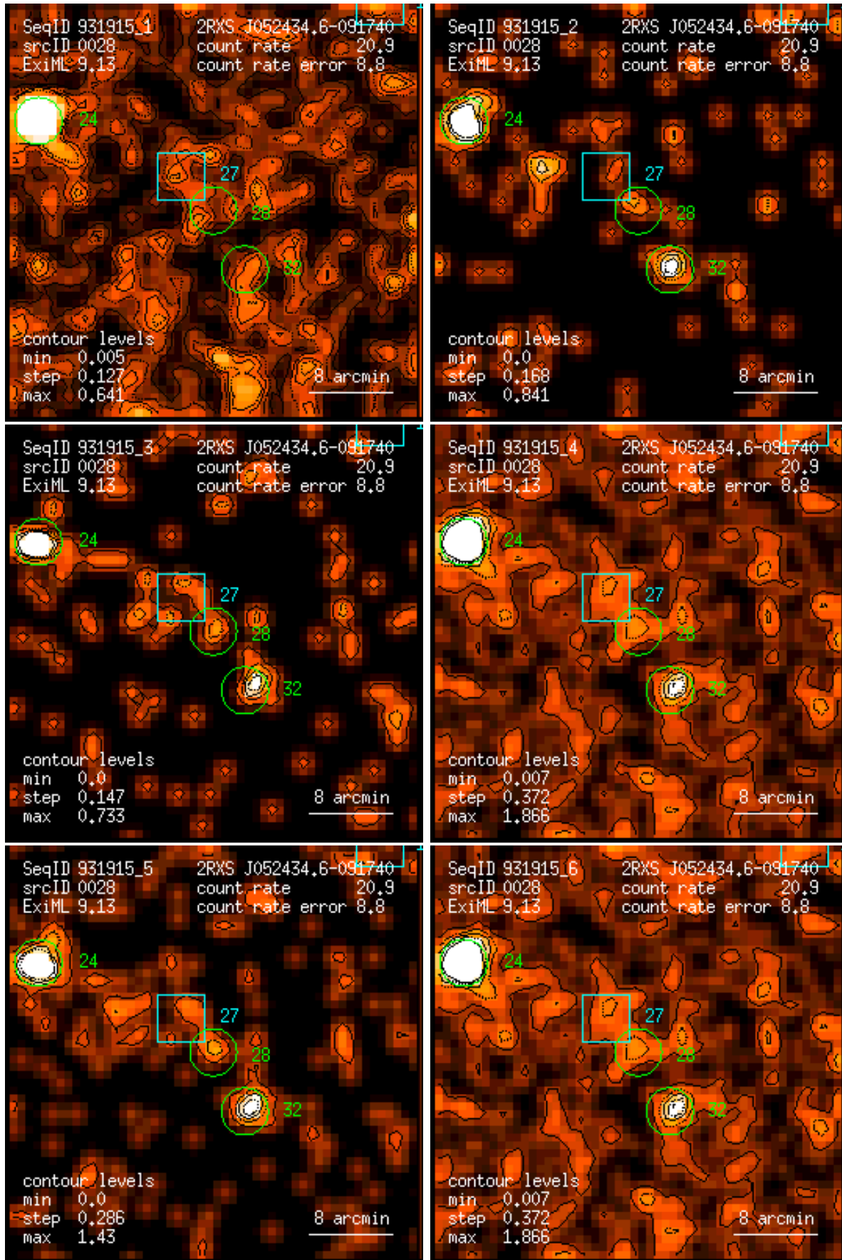
Figure 28: RASS 931915: detection 0028: band rate images, Gaussian filter: (1) PSPC channels 11 – 41, (2) 52 – 90, (3) 91 – 201, (4) 11 – 235, (5) 52 – 201, (6) 11 – 201. Broad band rates in counts/ks. Band rate contour levels in counts/ks/arcmin 2 .
