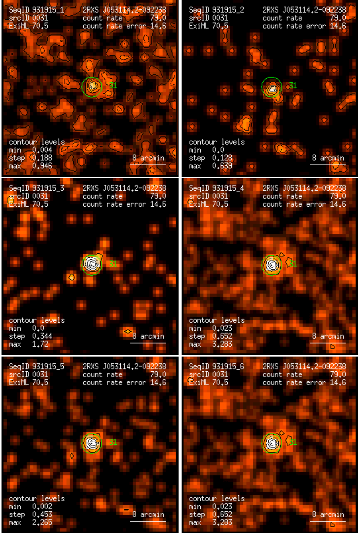
Figure 31: RASS 931915: detection 0031: band rate images, Gaussian filter: (1) PSPC channels 11 – 41, (2) 52 – 90, (3) 91 – 201, (4) 11 – 235, (5) 52 – 201, (6) 11 – 201. Broad band rates in counts/ks. Band rate contour levels in counts/ks/arcmin 2 .
