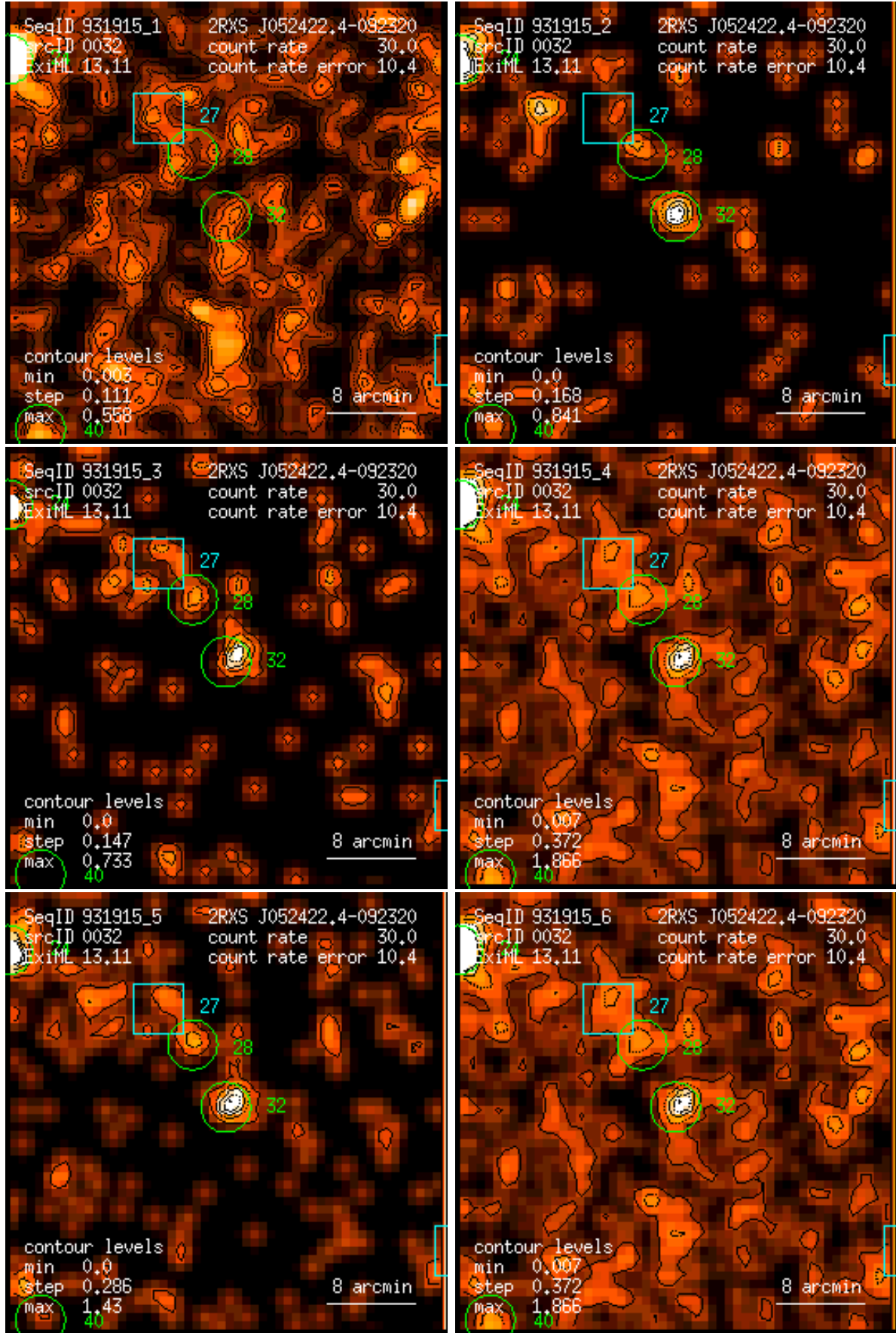
Figure 32: RASS 931915: detection 0032: band rate images, Gaussian filter: (1) PSPC channels 11 – 41, (2) 52 – 90, (3) 91 – 201, (4) 11 – 235, (5) 52 – 201, (6) 11 – 201. Broad band rates in counts/ks. Band rate contour levels in counts/ks/arcmin 2 .
