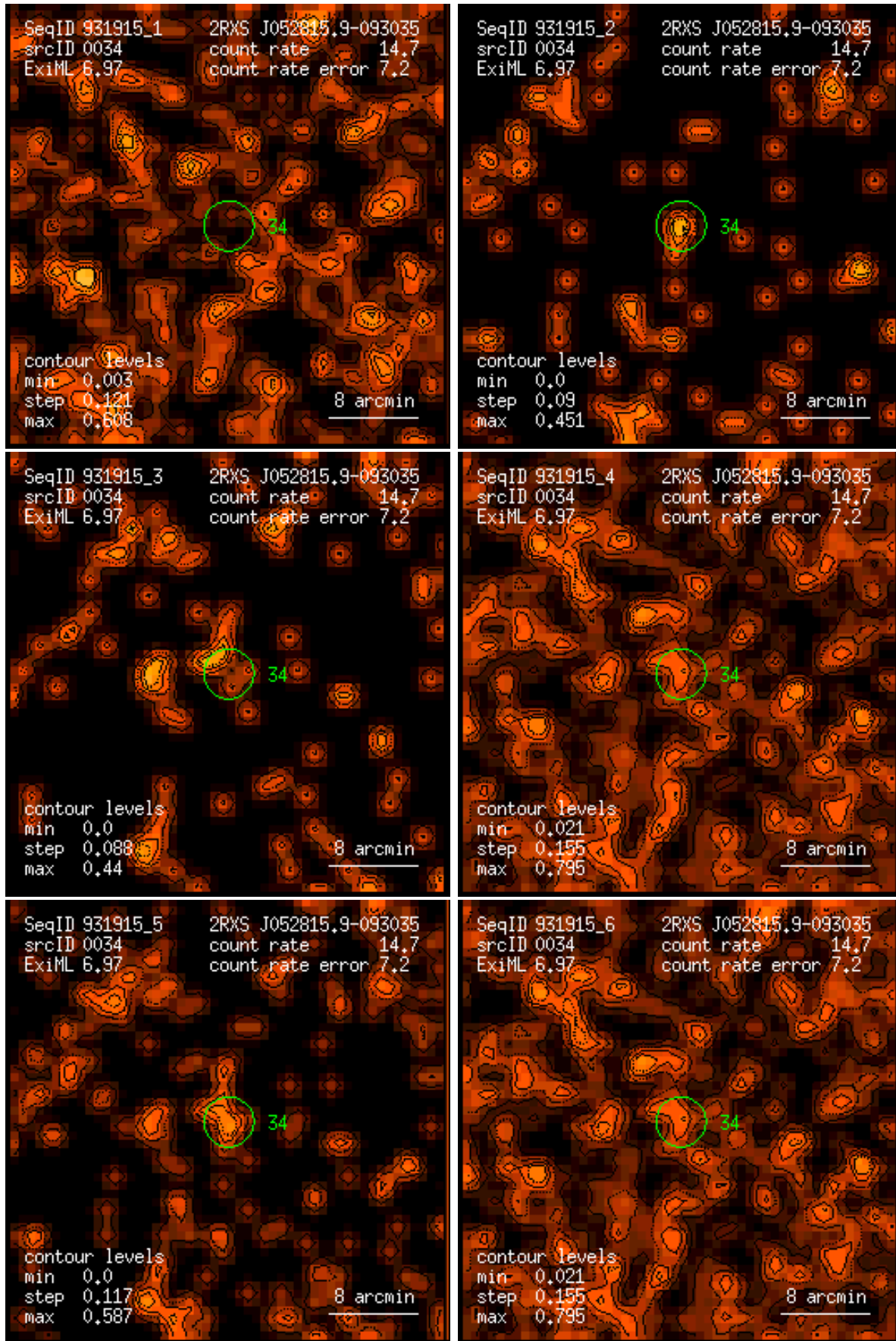
Figure 34: RASS 931915: detection 0034: band rate images, Gaussian filter: (1) PSPC channels 11 – 41, (2) 52 – 90, (3) 91 – 201, (4) 11 – 235, (5) 52 – 201, (6) 11 – 201. Broad band rates in counts/ks. Band rate contour levels in counts/ks/arcmin 2 .
