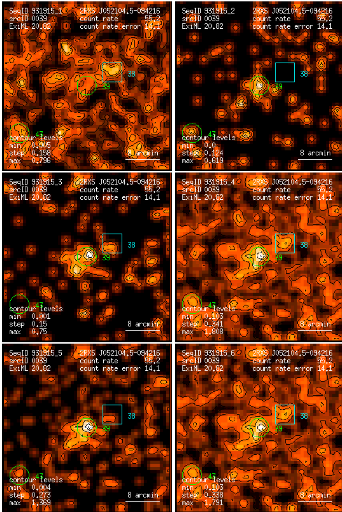
Figure 39: RASS 931915: detection 0039: band rate images, Gaussian filter: (1) PSPC channels 11 – 41, (2) 52 – 90, (3) 91 – 201, (4) 11 – 235, (5) 52 – 201, (6) 11 – 201. Broad band rates in counts/ks. Band rate contour levels in counts/ks/arcmin 2 .
