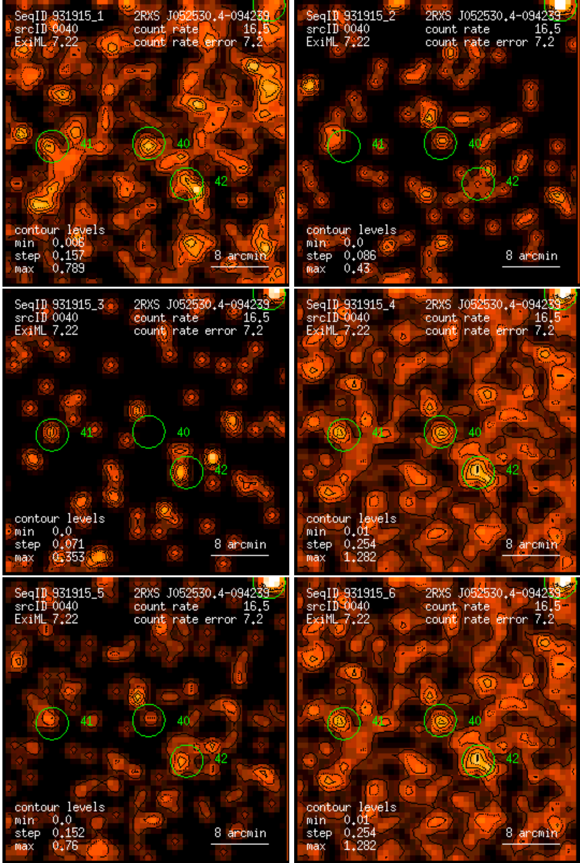
Figure 40: RASS 931915: detection 0040: band rate images, Gaussian filter: (1) PSPC channels 11 – 41, (2) 52 – 90, (3) 91 – 201, (4) 11 – 235, (5) 52 – 201, (6) 11 – 201. Broad band rates in counts/ks. Band rate contour levels in counts/ks/arcmin 2 .
