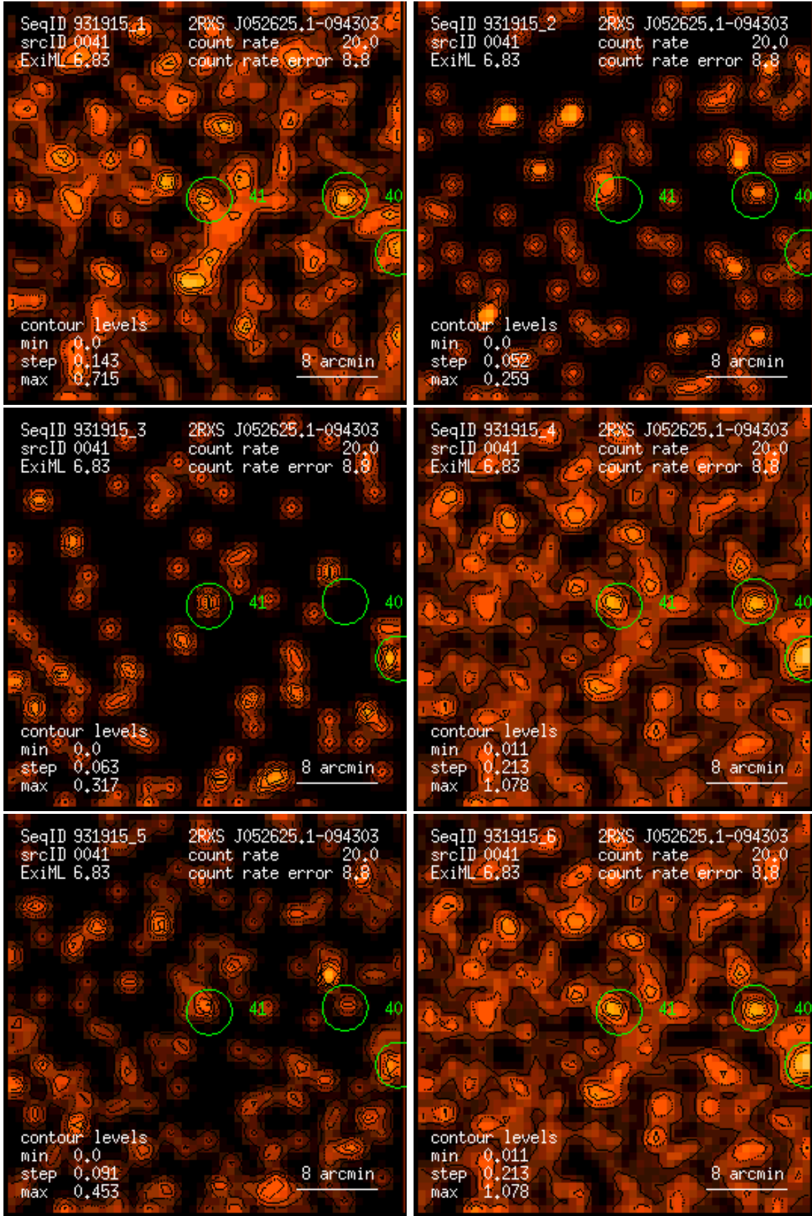
Figure 41: RASS 931915: detection 0041: band rate images, Gaussian filter: (1) PSPC channels 11 – 41, (2) 52 – 90, (3) 91 – 201, (4) 11 – 235, (5) 52 – 201, (6) 11 – 201. Broad band rates in counts/ks. Band rate contour levels in counts/ks/arcmin 2 .
