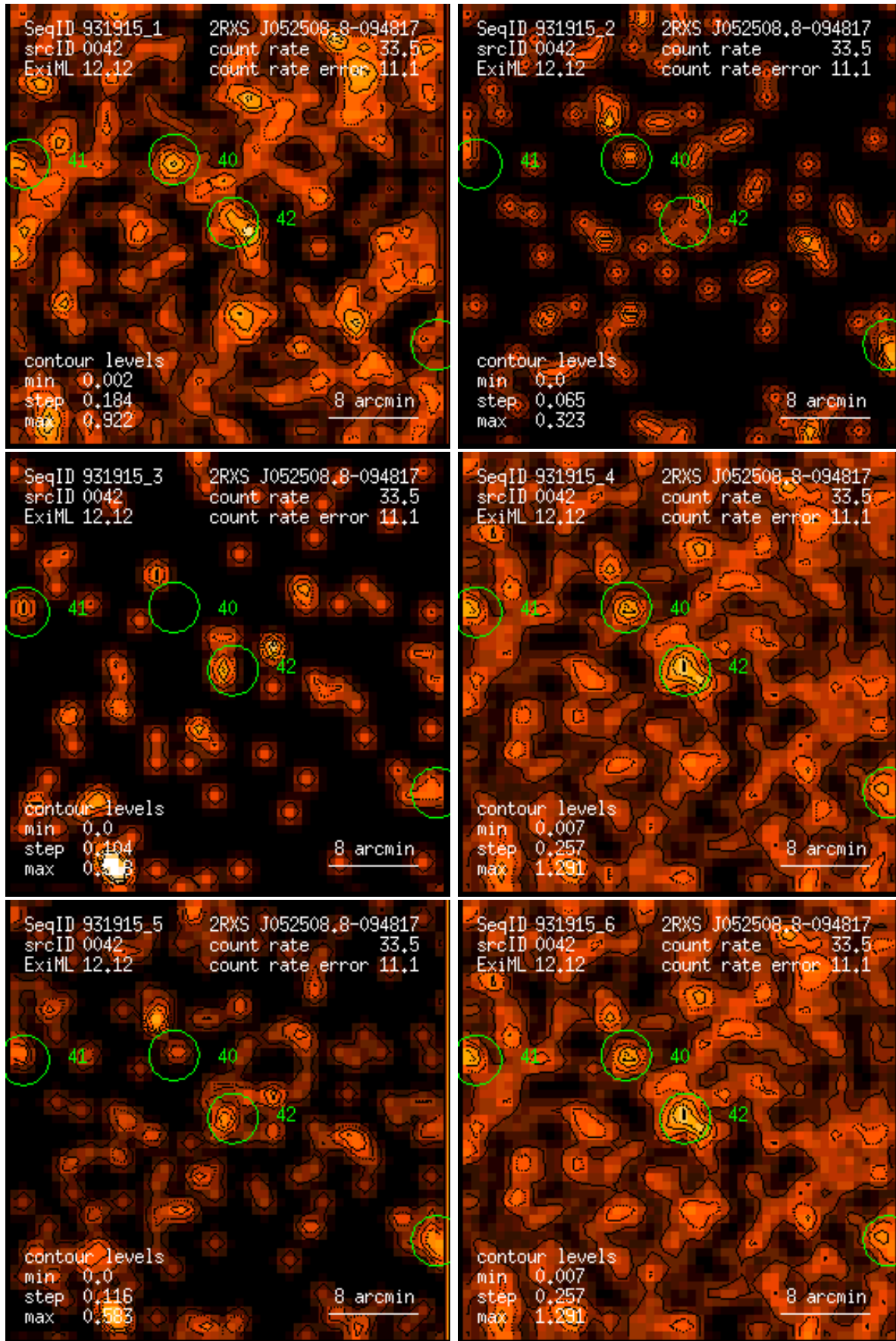
Figure 42: RASS 931915: detection 0042: band rate images, Gaussian filter: (1) PSPC channels 11 – 41, (2) 52 – 90, (3) 91 – 201, (4) 11 – 235, (5) 52 – 201, (6) 11 – 201. Broad band rates in counts/ks. Band rate contour levels in counts/ks/arcmin 2 .
