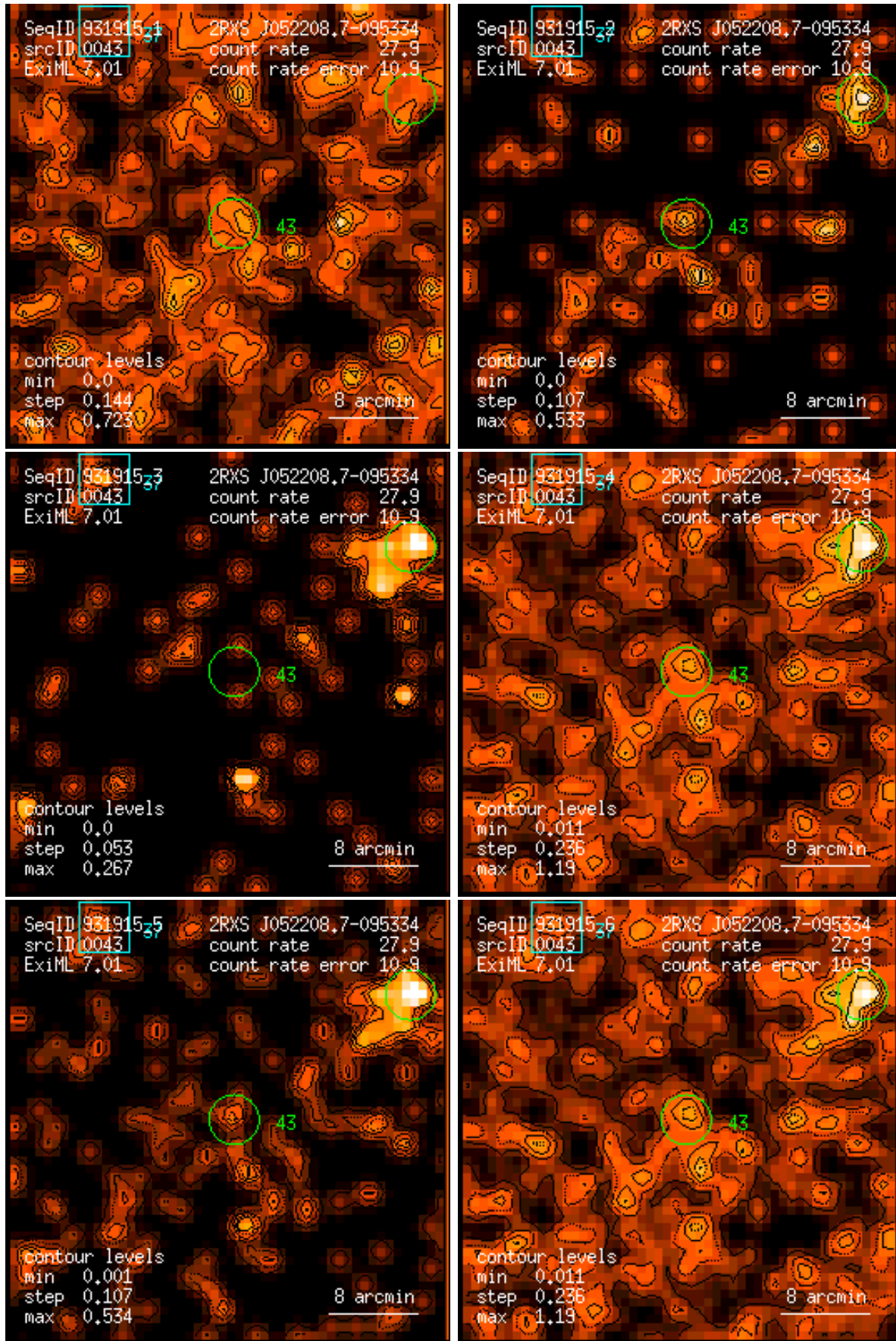
Figure 43: RASS 931915: detection 0043: band rate images, Gaussian filter: (1) PSPC channels 11 – 41, (2) 52 – 90, (3) 91 – 201, (4) 11 – 235, (5) 52 – 201, (6) 11 – 201. Broad band rates in counts/ks. Band rate contour levels in counts/ks/arcmin 2 .
