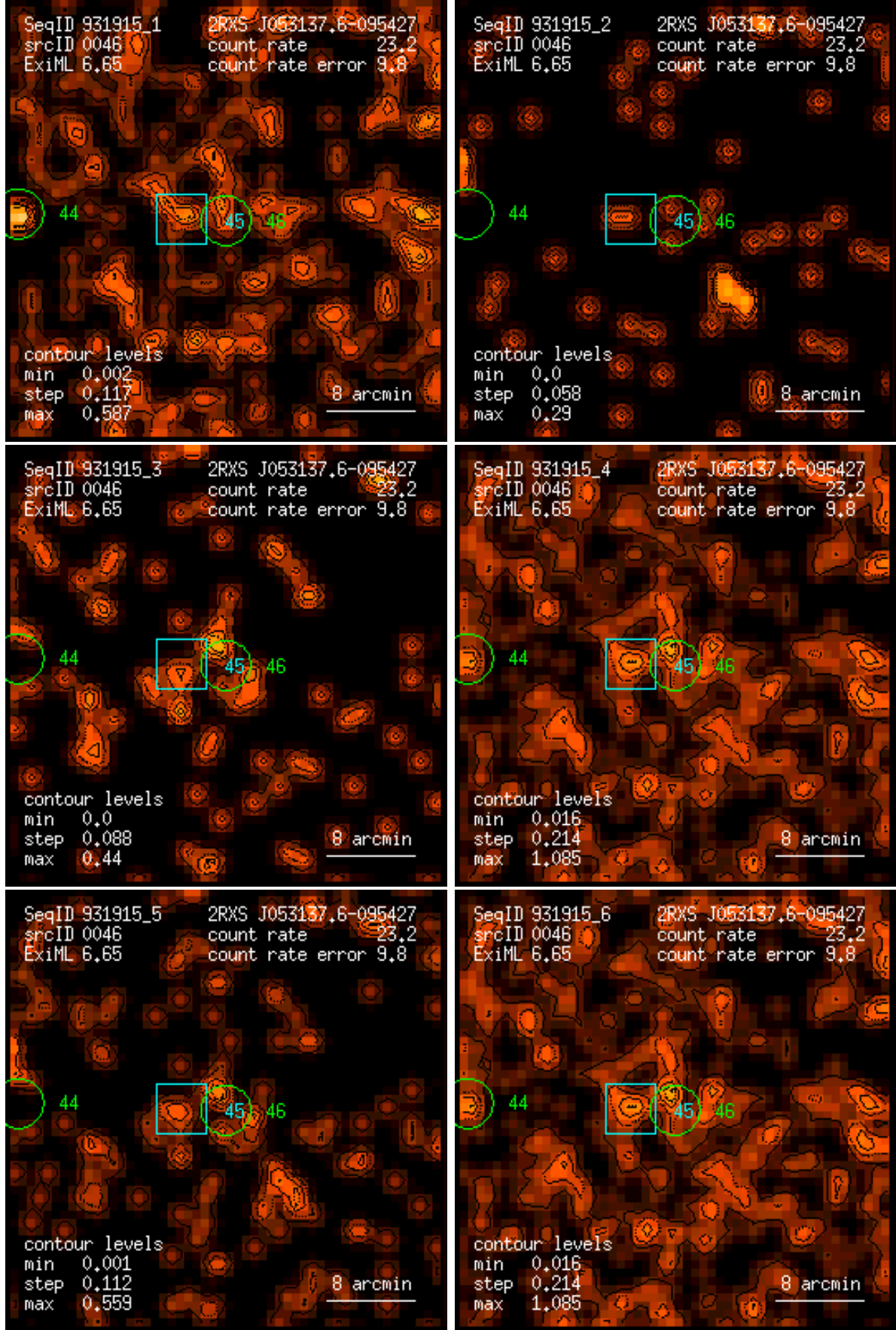
Figure 46: RASS 931915: detection 0046: band rate images, Gaussian filter: (1) PSPC channels 11 – 41, (2) 52 – 90, (3) 91 – 201, (4) 11 – 235, (5) 52 – 201, (6) 11 – 201. Broad band rates in counts/ks. Band rate contour levels in counts/ks/arcmin 2 .
