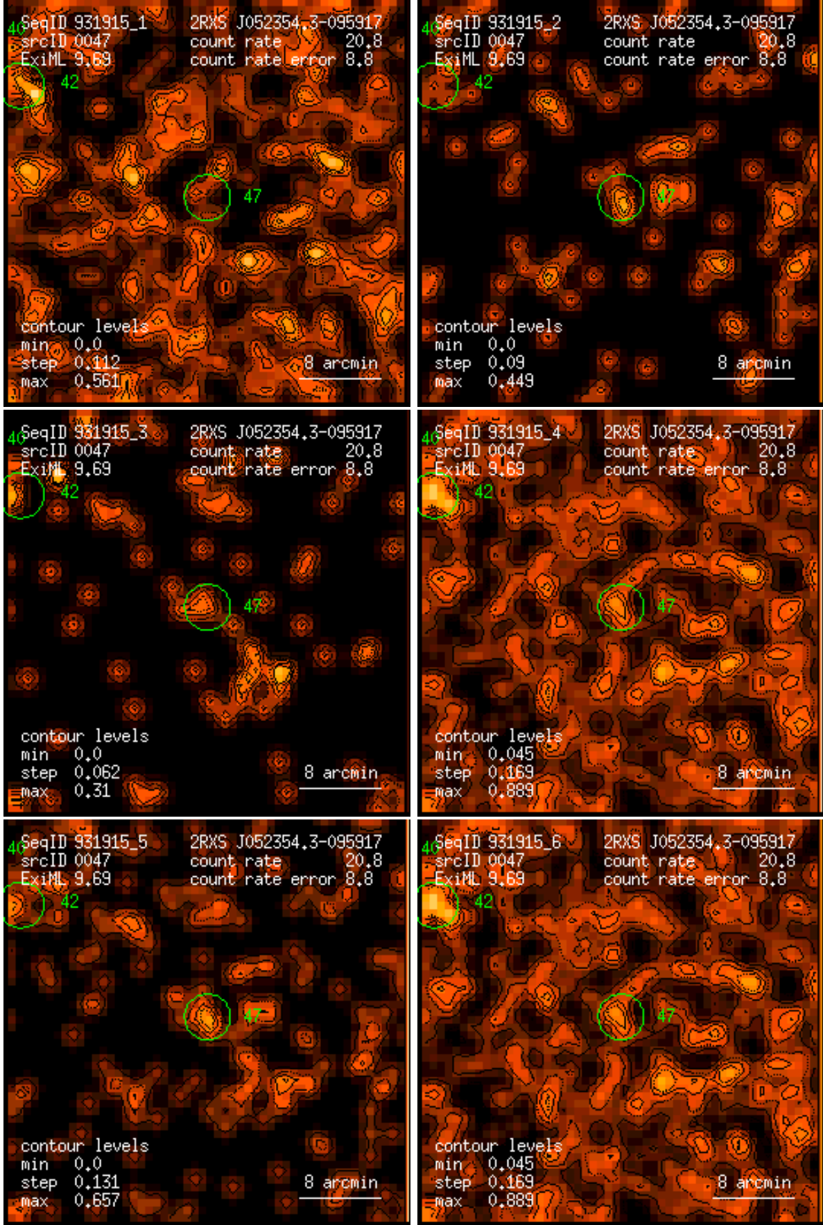
Figure 47: RASS 931915: detection 0047: band rate images, Gaussian filter: (1) PSPC channels 11 – 41, (2) 52 – 90, (3) 91 – 201, (4) 11 – 235, (5) 52 – 201, (6) 11 – 201. Broad band rates in counts/ks. Band rate contour levels in counts/ks/arcmin 2 .
