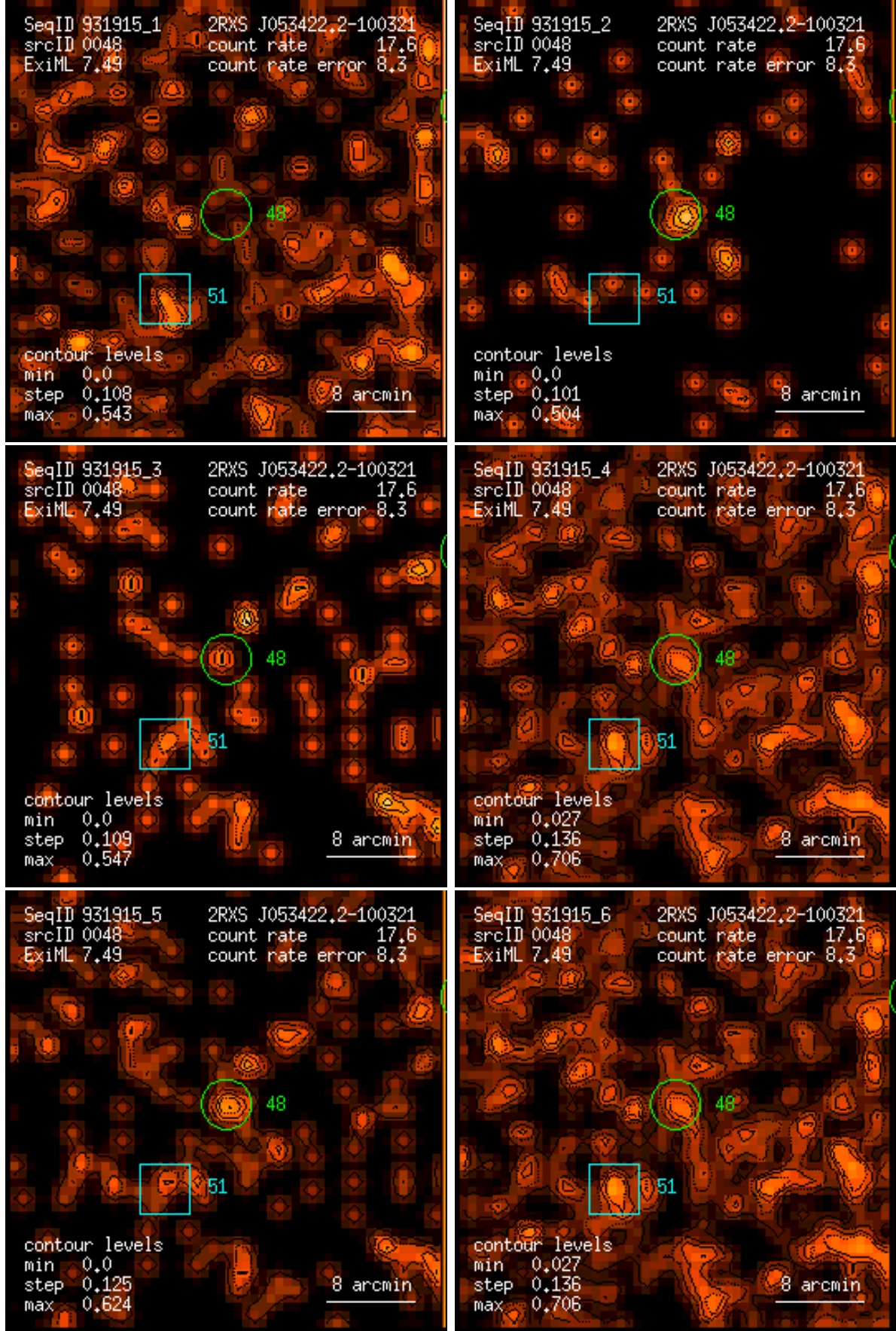
Figure 48: RASS 931915: detection 0048: band rate images, Gaussian filter: (1) PSPC channels 11 – 41, (2) 52 – 90, (3) 91 – 201, (4) 11 – 235, (5) 52 – 201, (6) 11 – 201. Broad band rates in counts/ks. Band rate contour levels in counts/ks/arcmin 2 .
