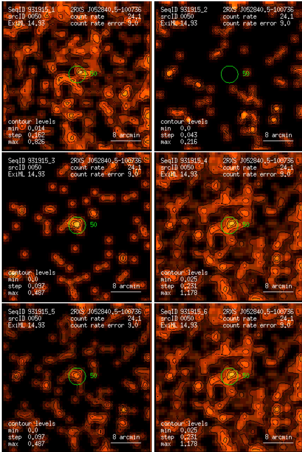
Figure 50: RASS 931915: detection 0050: band rate images, Gaussian filter: (1) PSPC channels 11 – 41, (2) 52 – 90, (3) 91 – 201, (4) 11 – 235, (5) 52 – 201, (6) 11 – 201. Broad band rates in counts/ks. Band rate contour levels in counts/ks/arcmin 2 .
