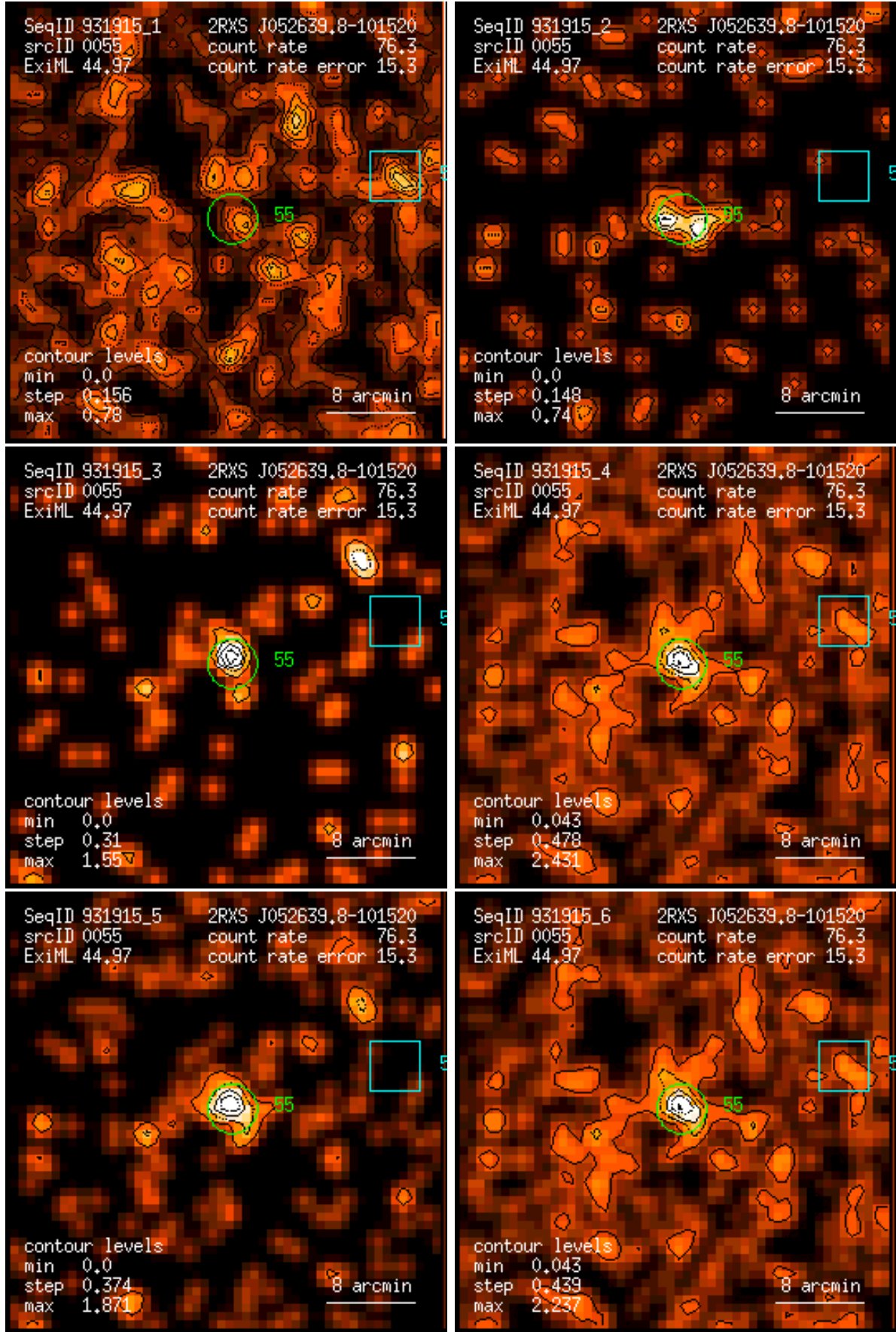
Figure 55: RASS 931915: detection 0055: band rate images, Gaussian filter: (1) PSPC channels 11 – 41, (2) 52 – 90, (3) 91 – 201, (4) 11 – 235, (5) 52 – 201, (6) 11 – 201. Broad band rates in counts/ks. Band rate contour levels in counts/ks/arcmin 2 .
