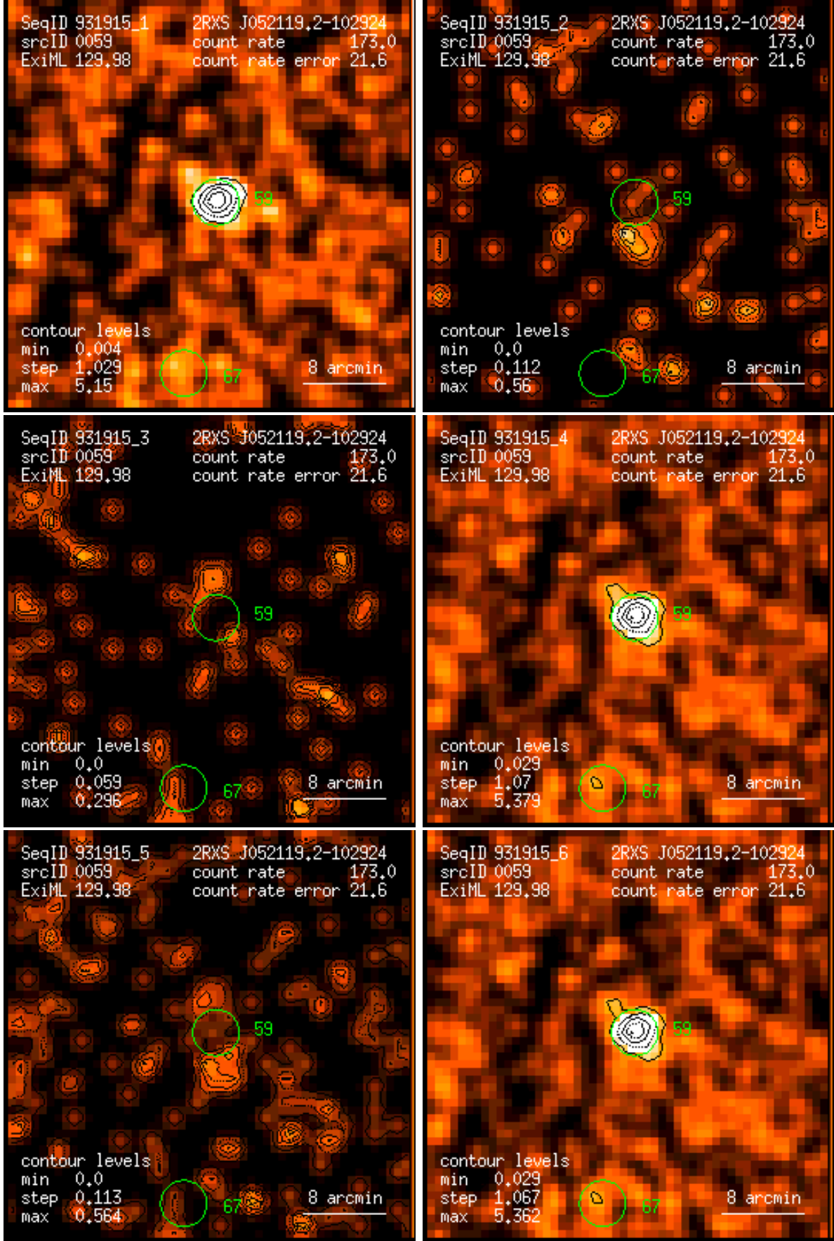
Figure 59: RASS 931915: detection 0059: band rate images, Gaussian filter: (1) PSPC channels 11 – 41, (2) 52 – 90, (3) 91 – 201, (4) 11 – 235, (5) 52 – 201, (6) 11 – 201. Broad band rates in counts/ks. Band rate contour levels in counts/ks/arcmin 2 .
