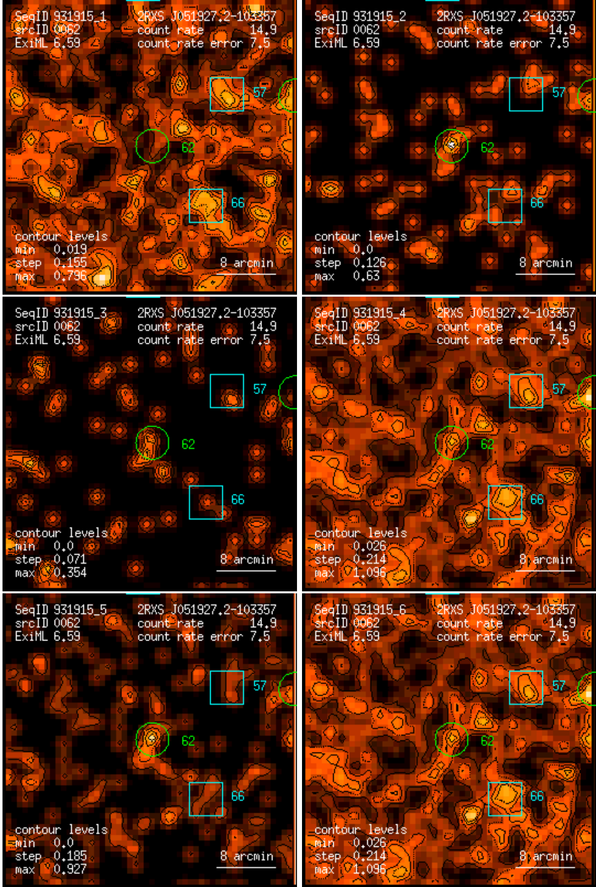
Figure 62: RASS 931915: detection 0062: band rate images, Gaussian filter: (1) PSPC channels 11 – 41, (2) 52 – 90, (3) 91 – 201, (4) 11 – 235, (5) 52 – 201, (6) 11 – 201. Broad band rates in counts/ks. Band rate contour levels in counts/ks/arcmin 2 .
