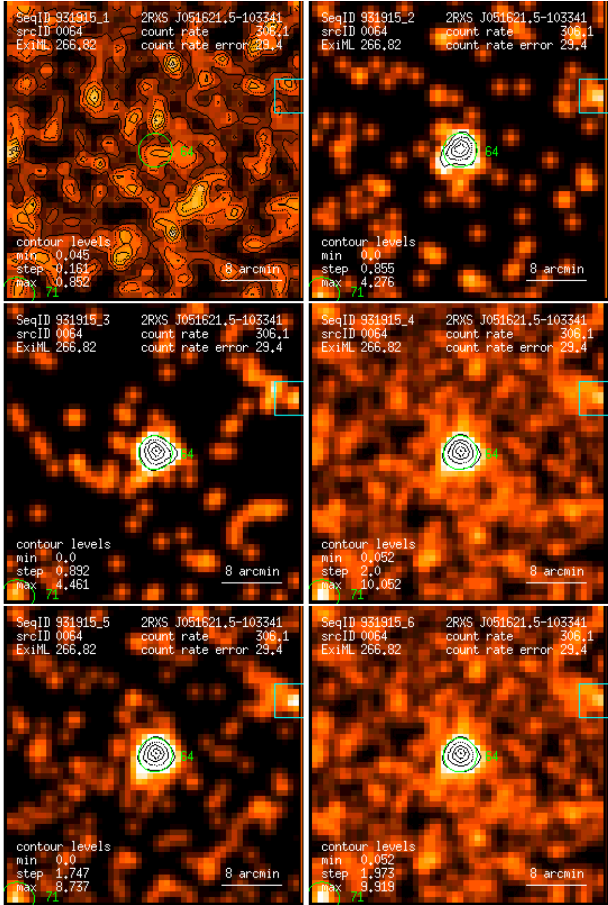
Figure 64: RASS 931915: detection 0064: band rate images, Gaussian filter: (1) PSPC channels 11 – 41, (2) 52 – 90, (3) 91 – 201, (4) 11 – 235, (5) 52 – 201, (6) 11 – 201. Broad band rates in counts/ks. Band rate contour levels in counts/ks/arcmin 2 .
