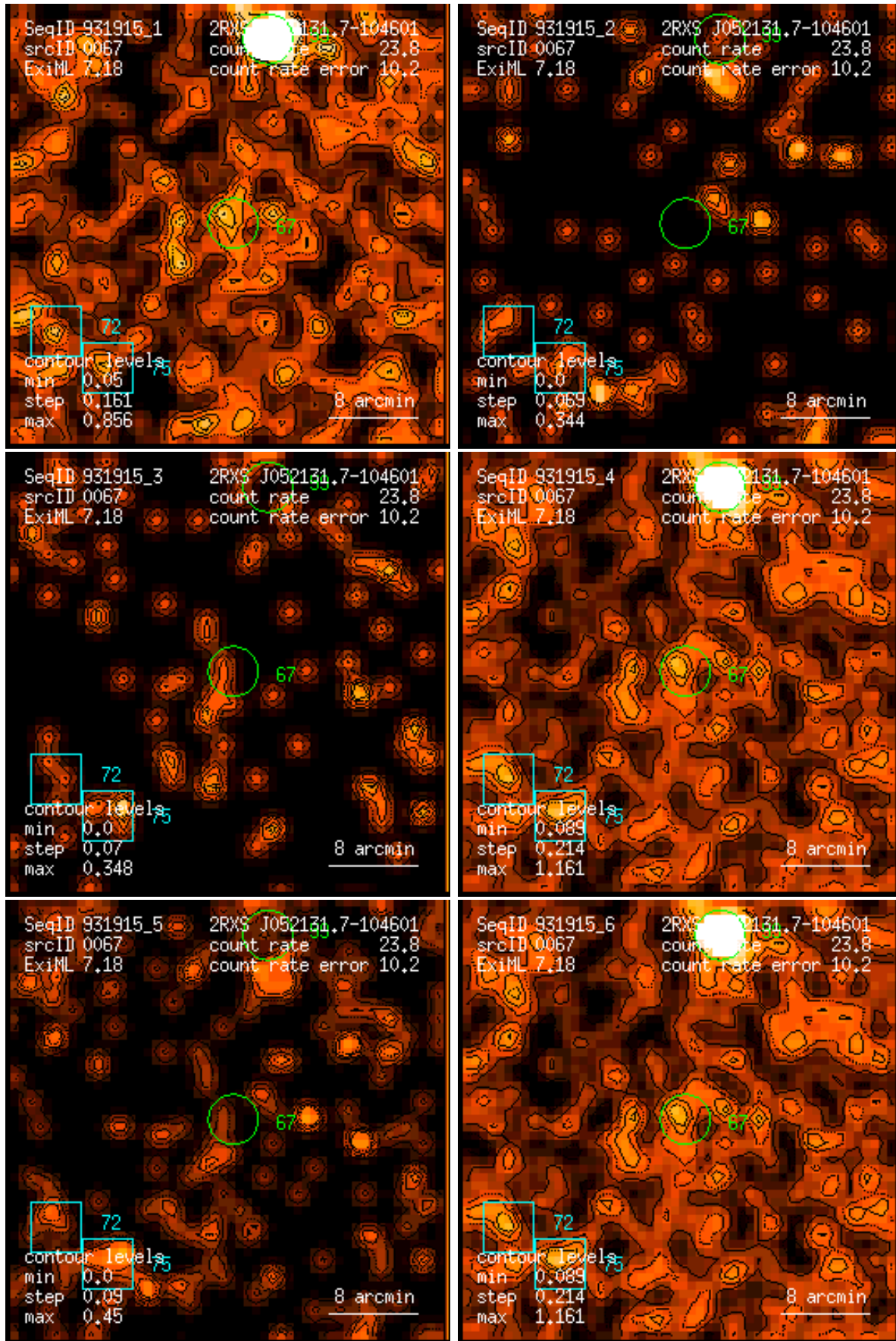
Figure 67: RASS 931915: detection 0067: band rate images, Gaussian filter: (1) PSPC channels 11 – 41, (2) 52 – 90, (3) 91 – 201, (4) 11 – 235, (5) 52 – 201, (6) 11 – 201. Broad band rates in counts/ks. Band rate contour levels in counts/ks/arcmin 2 .
