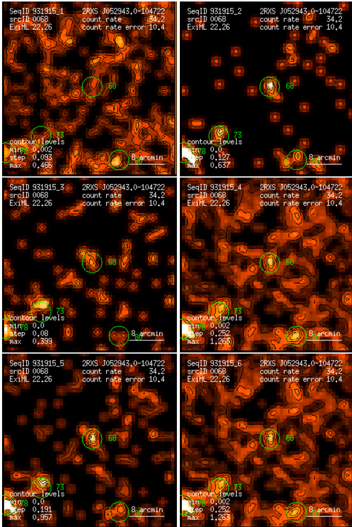
Figure 68: RASS 931915: detection 0068: band rate images, Gaussian filter: (1) PSPC channels 11 – 41, (2) 52 – 90, (3) 91 – 201, (4) 11 – 235, (5) 52 – 201, (6) 11 – 201. Broad band rates in counts/ks. Band rate contour levels in counts/ks/arcmin 2 .
