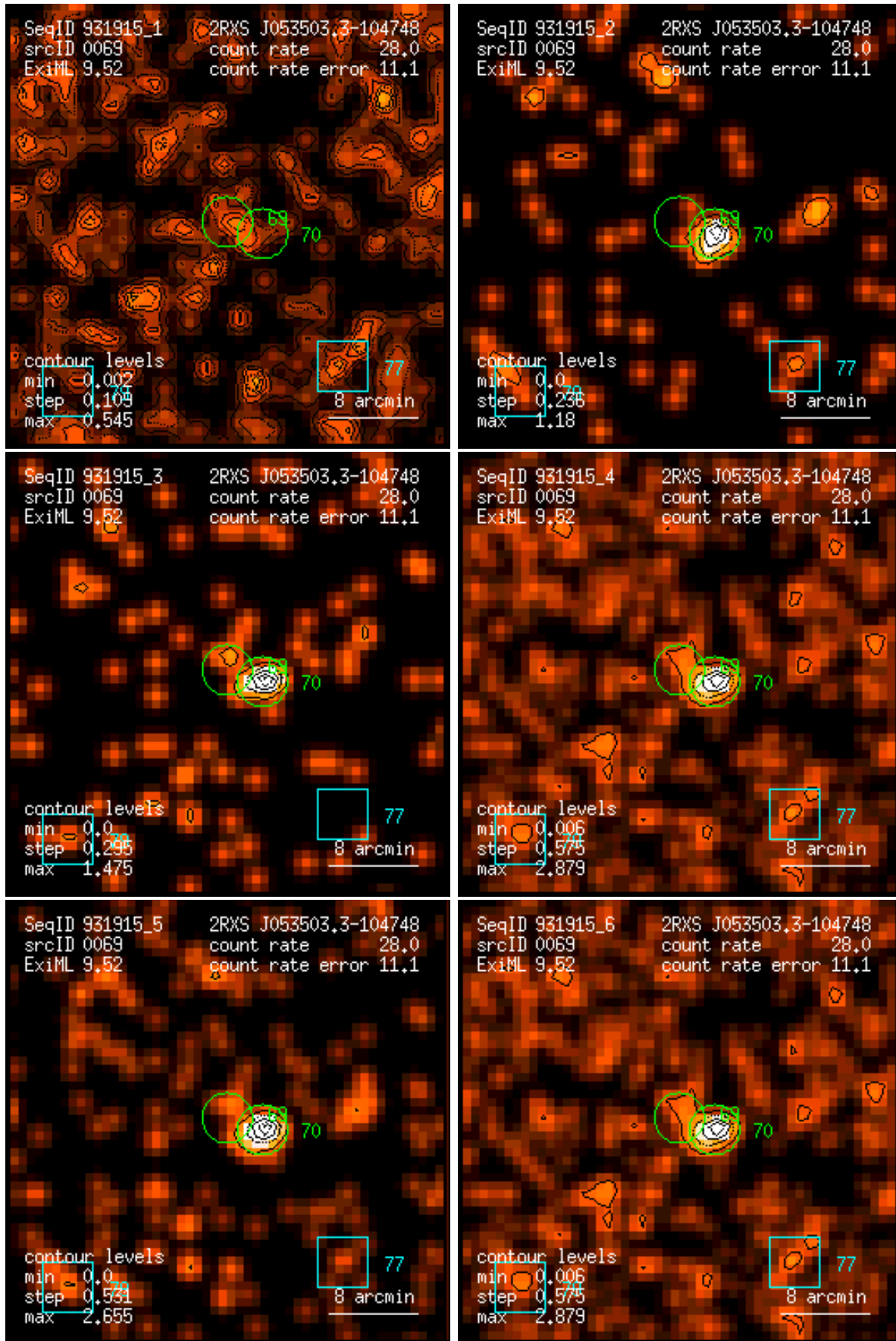
Figure 69: RASS 931915: detection 0069: band rate images, Gaussian filter: (1) PSPC channels 11 – 41, (2) 52 – 90, (3) 91 – 201, (4) 11 – 235, (5) 52 – 201, (6) 11 – 201. Broad band rates in counts/ks. Band rate contour levels in counts/ks/arcmin 2 .
