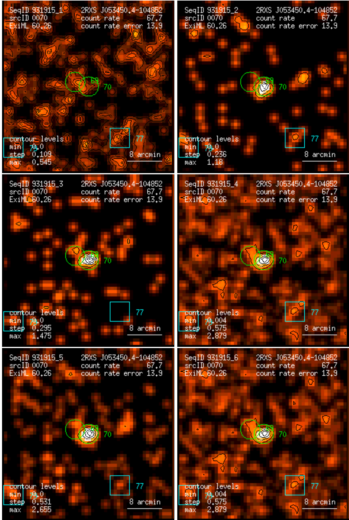
Figure 70: RASS 931915: detection 0070: band rate images, Gaussian filter: (1) PSPC channels 11 – 41, (2) 52 – 90, (3) 91 – 201, (4) 11 – 235, (5) 52 – 201, (6) 11 – 201. Broad band rates in counts/ks. Band rate contour levels in counts/ks/arcmin 2 .
