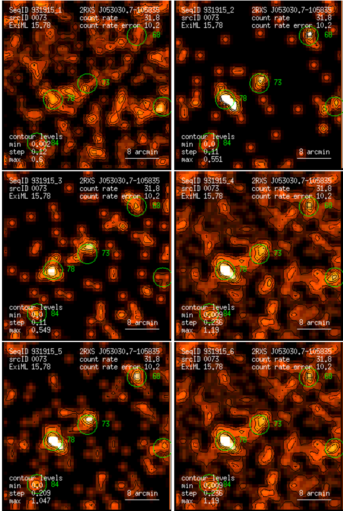
Figure 73: RASS 931915: detection 0073: band rate images, Gaussian filter: (1) PSPC channels 11 – 41, (2) 52 – 90, (3) 91 – 201, (4) 11 – 235, (5) 52 – 201, (6) 11 – 201. Broad band rates in counts/ks. Band rate contour levels in counts/ks/arcmin 2 .
