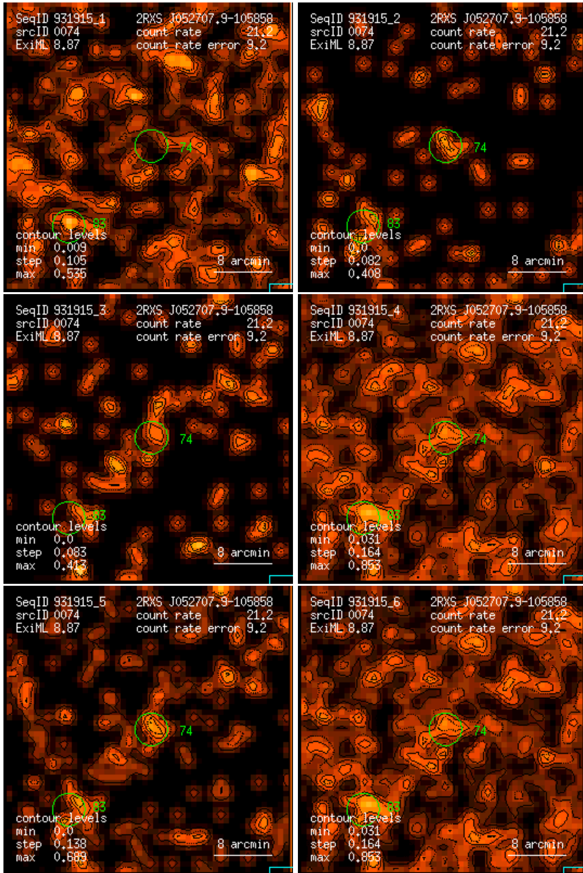
Figure 74: RASS 931915: detection 0074: band rate images, Gaussian filter: (1) PSPC channels 11 – 41, (2) 52 – 90, (3) 91 – 201, (4) 11 – 235, (5) 52 – 201, (6) 11 – 201. Broad band rates in counts/ks. Band rate contour levels in counts/ks/arcmin 2 .
