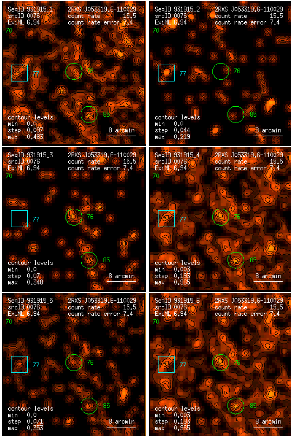
Figure 76: RASS 931915: detection 0076: band rate images, Gaussian filter: (1) PSPC channels 11 – 41, (2) 52 – 90, (3) 91 – 201, (4) 11 – 235, (5) 52 – 201, (6) 11 – 201. Broad band rates in counts/ks. Band rate contour levels in counts/ks/arcmin 2 .
