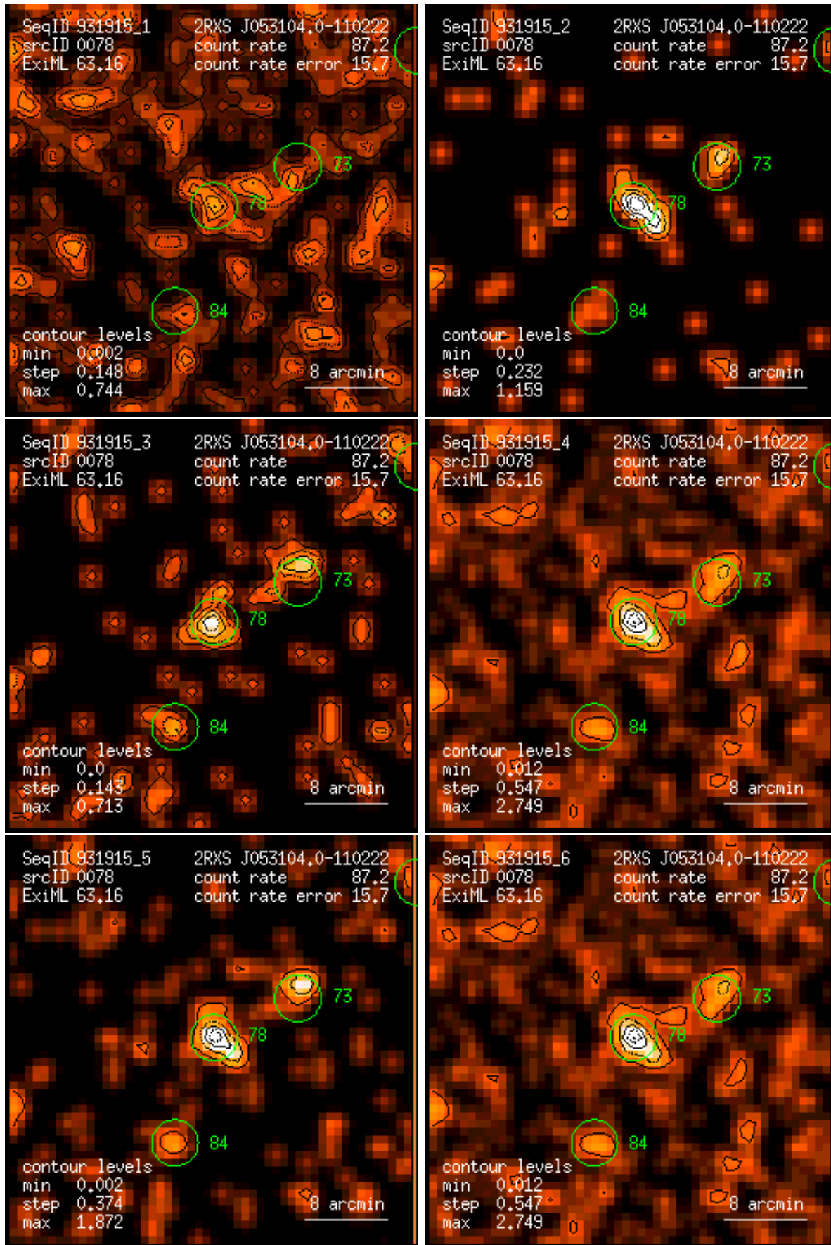
Figure 78: RASS 931915: detection 0078: band rate images, Gaussian filter: (1) PSPC channels 11 – 41, (2) 52 – 90, (3) 91 – 201, (4) 11 – 235, (5) 52 – 201, (6) 11 – 201. Broad band rates in counts/ks. Band rate contour levels in counts/ks/arcmin 2 .
