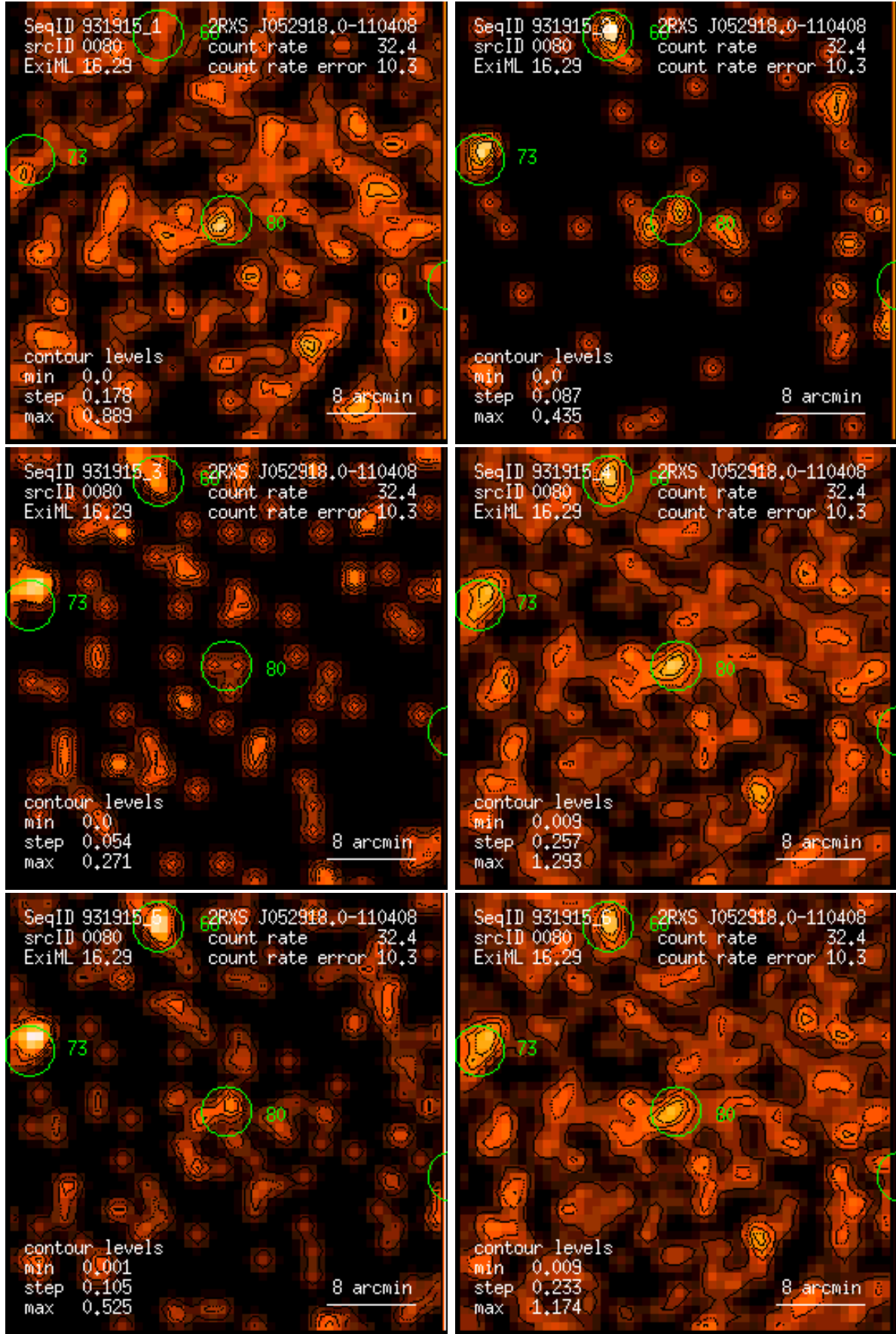
Figure 80: RASS 931915: detection 0080: band rate images, Gaussian filter: (1) PSPC channels 11 – 41, (2) 52 – 90, (3) 91 – 201, (4) 11 – 235, (5) 52 – 201, (6) 11 – 201. Broad band rates in counts/ks. Band rate contour levels in counts/ks/arcmin 2 .
