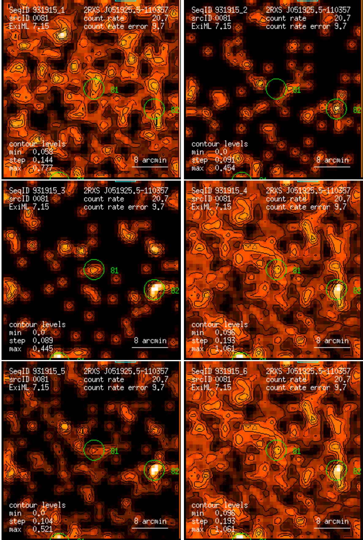
Figure 81: RASS 931915: detection 0081: band rate images, Gaussian filter: (1) PSPC channels 11 – 41, (2) 52 – 90, (3) 91 – 201, (4) 11 – 235, (5) 52 – 201, (6) 11 – 201. Broad band rates in counts/ks. Band rate contour levels in counts/ks/arcmin 2 .
