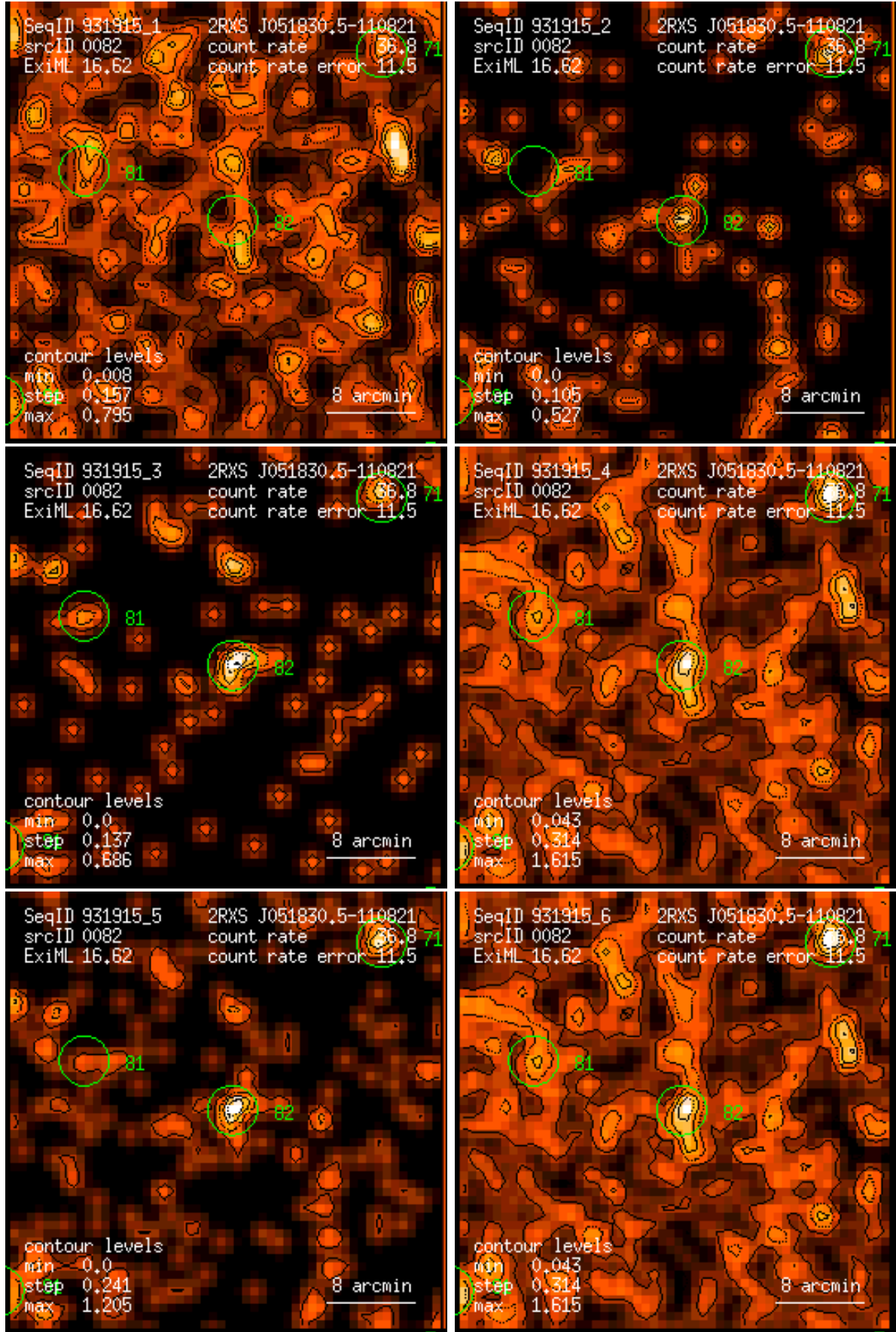
Figure 82: RASS 931915: detection 0082: band rate images, Gaussian filter: (1) PSPC channels 11 – 41, (2) 52 – 90, (3) 91 – 201, (4) 11 – 235, (5) 52 – 201, (6) 11 – 201. Broad band rates in counts/ks. Band rate contour levels in counts/ks/arcmin 2 .
