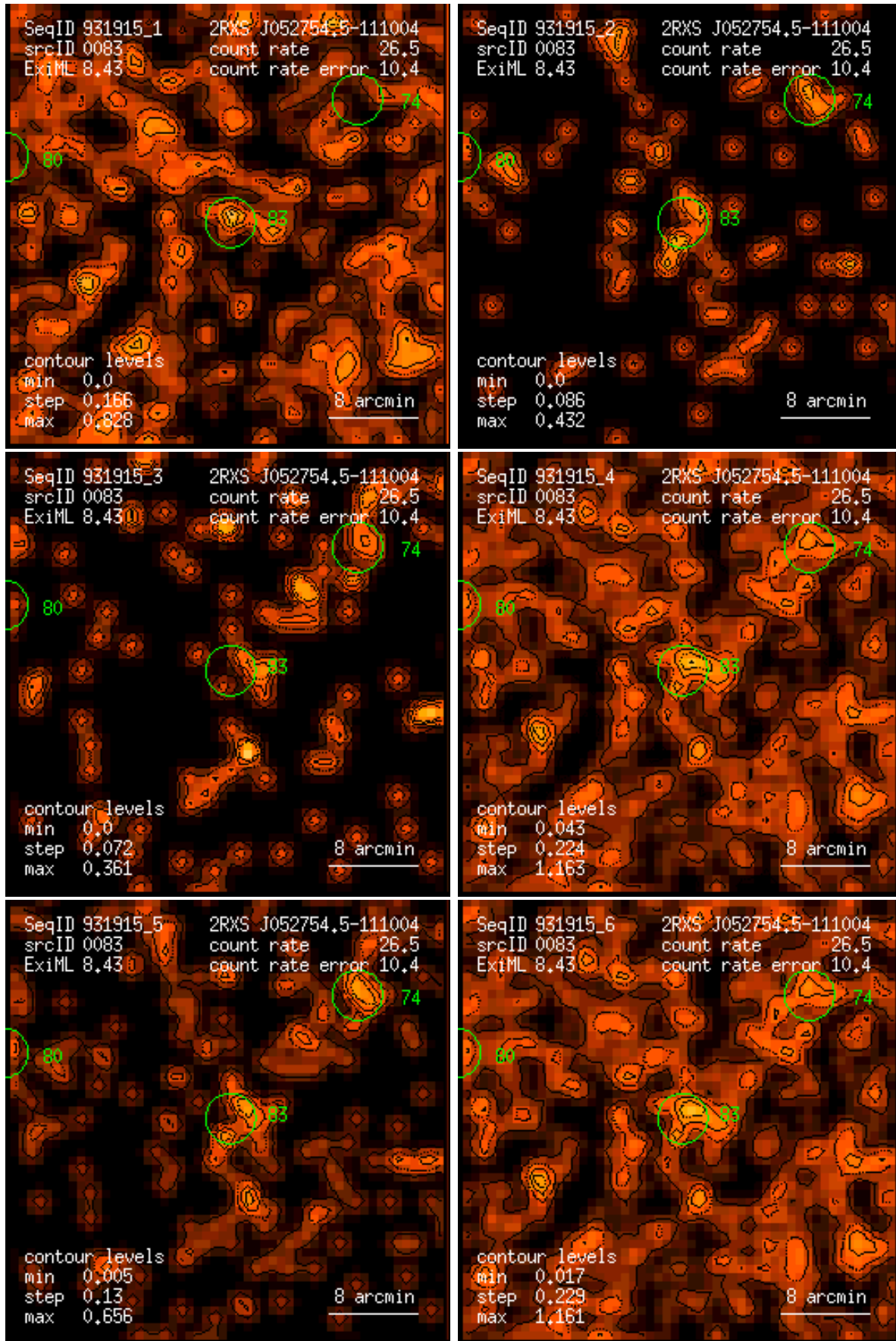
Figure 83: RASS 931915: detection 0083: band rate images, Gaussian filter: (1) PSPC channels 11 – 41, (2) 52 – 90, (3) 91 – 201, (4) 11 – 235, (5) 52 – 201, (6) 11 – 201. Broad band rates in counts/ks. Band rate contour levels in counts/ks/arcmin 2 .
