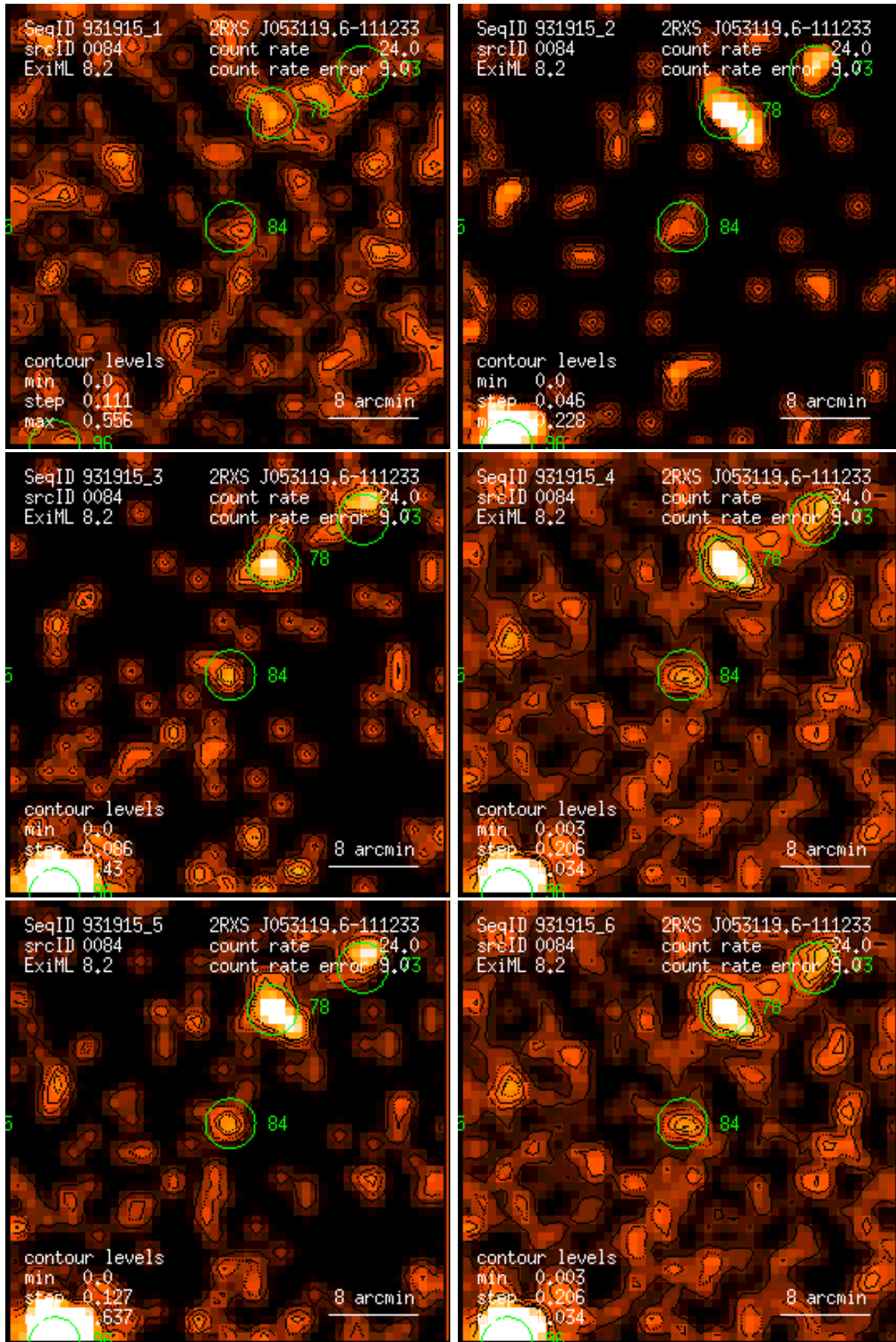
Figure 84: RASS 931915: detection 0084: band rate images, Gaussian filter: (1) PSPC channels 11 – 41, (2) 52 – 90, (3) 91 – 201, (4) 11 – 235, (5) 52 – 201, (6) 11 – 201. Broad band rates in counts/ks. Band rate contour levels in counts/ks/arcmin 2 .
