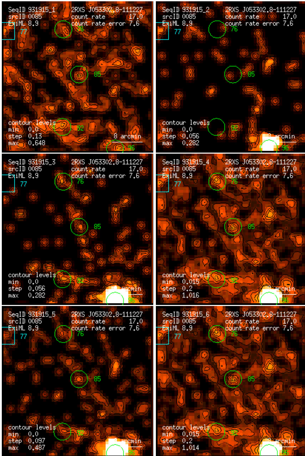
Figure 85: RASS 931915: detection 0085: band rate images, Gaussian filter: (1) PSPC channels 11 – 41, (2) 52 – 90, (3) 91 – 201, (4) 11 – 235, (5) 52 – 201, (6) 11 – 201. Broad band rates in counts/ks. Band rate contour levels in counts/ks/arcmin 2 .
