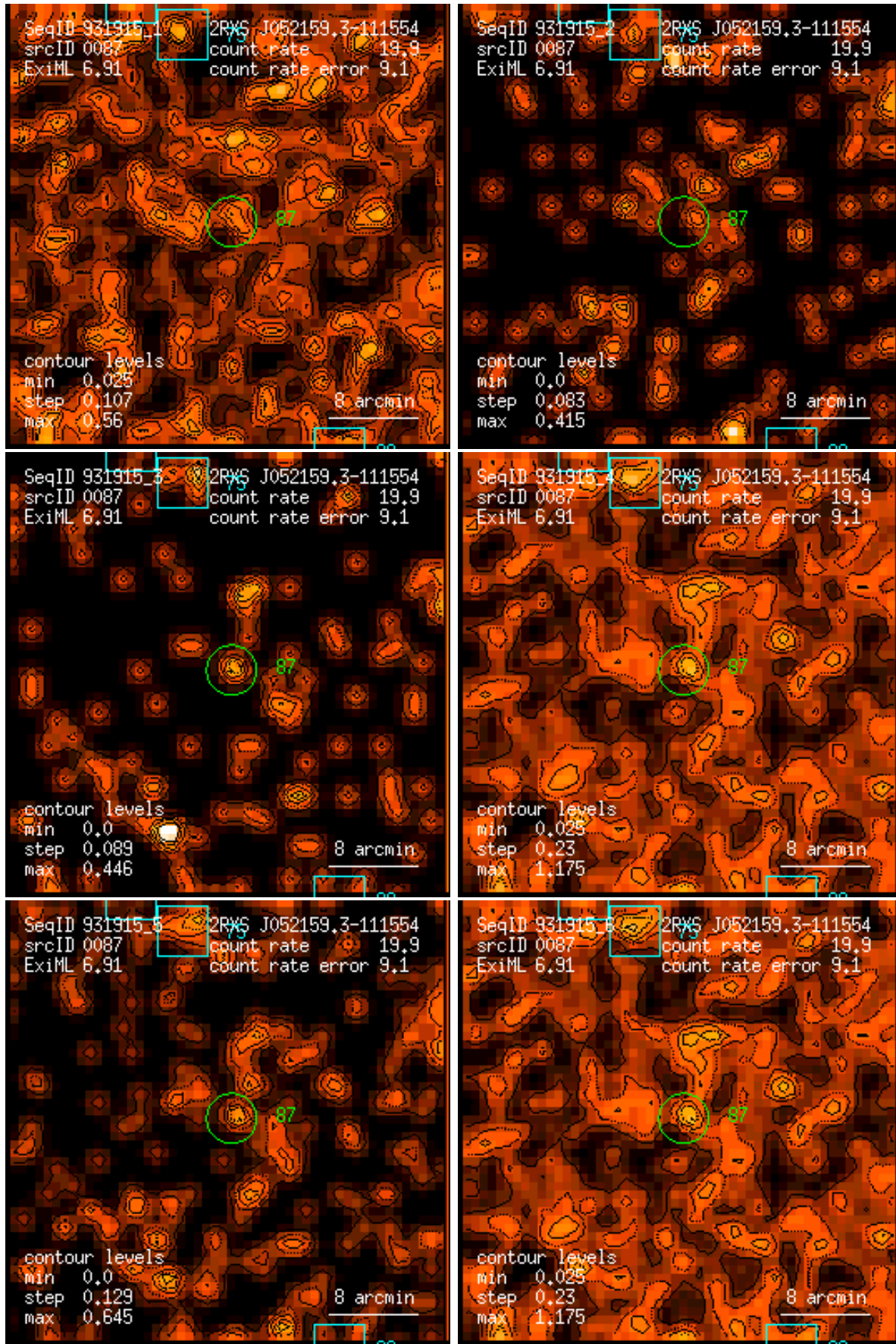
Figure 87: RASS 931915: detection 0087: band rate images, Gaussian filter: (1) PSPC channels 11 – 41, (2) 52 – 90, (3) 91 – 201, (4) 11 – 235, (5) 52 – 201, (6) 11 – 201. Broad band rates in counts/ks. Band rate contour levels in counts/ks/arcmin 2 .
