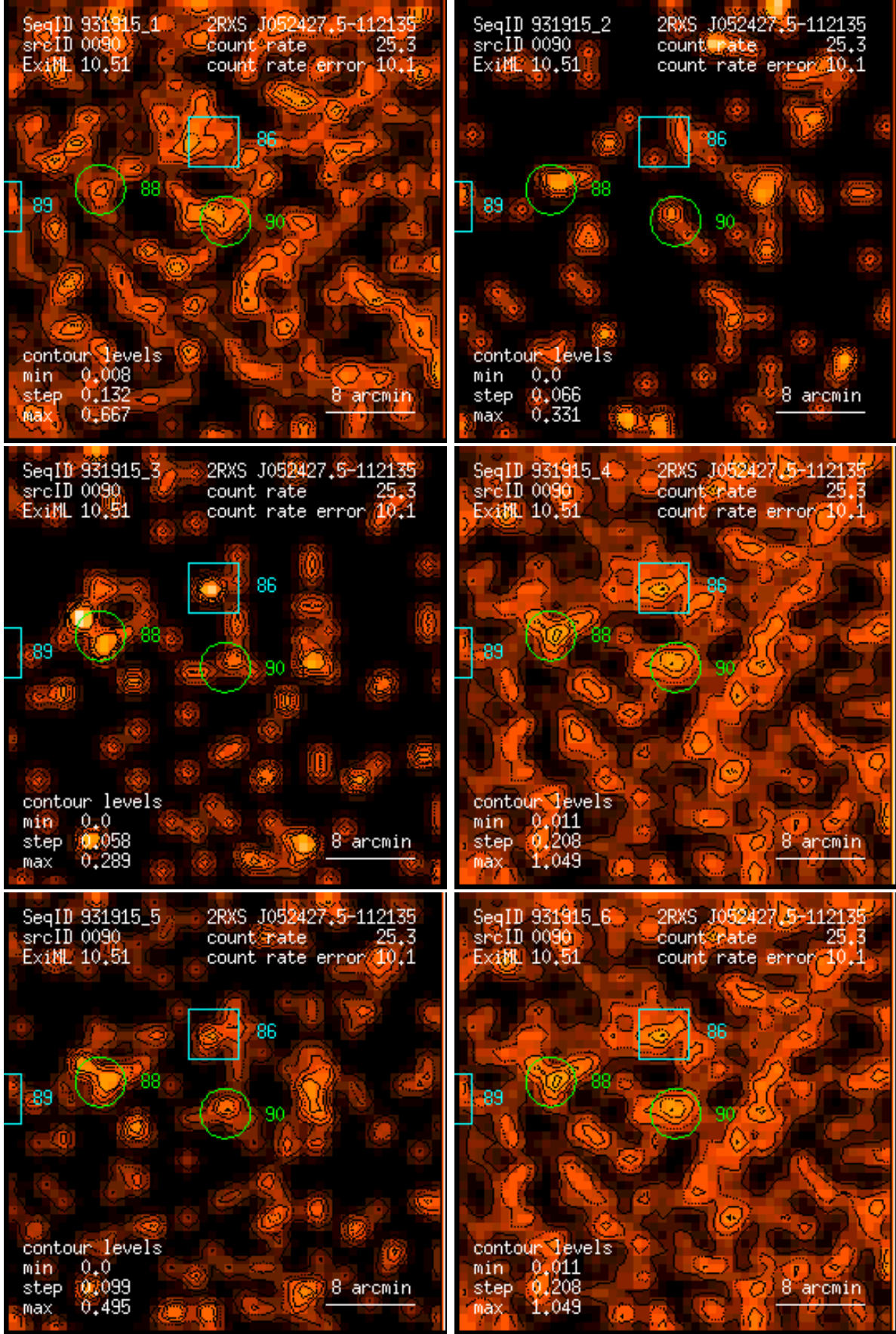
Figure 90: RASS 931915: detection 0090: band rate images, Gaussian filter: (1) PSPC channels 11 – 41, (2) 52 – 90, (3) 91 – 201, (4) 11 – 235, (5) 52 – 201, (6) 11 – 201. Broad band rates in counts/ks. Band rate contour levels in counts/ks/arcmin 2 .
