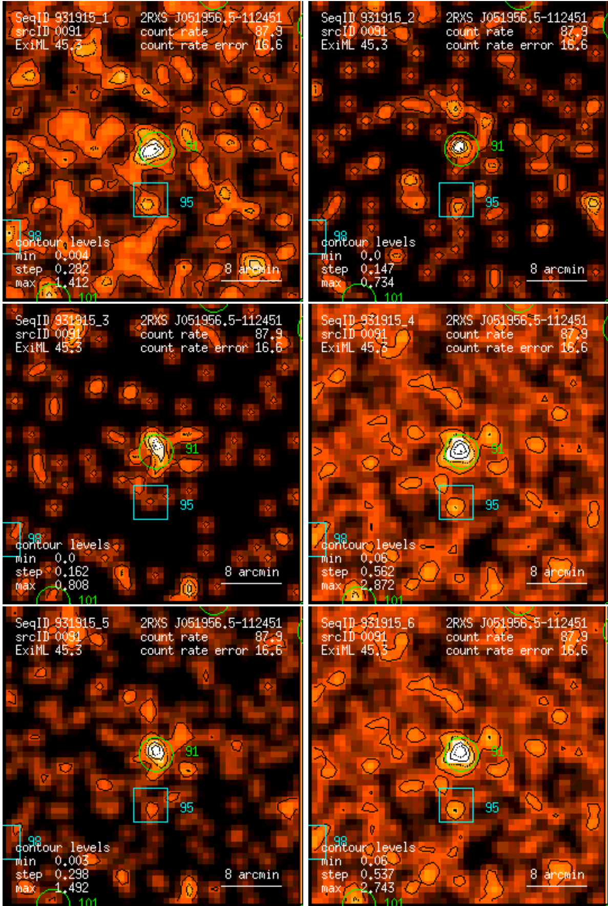
Figure 91: RASS 931915: detection 0091: band rate images, Gaussian filter: (1) PSPC channels 11 – 41, (2) 52 – 90, (3) 91 – 201, (4) 11 – 235, (5) 52 – 201, (6) 11 – 201. Broad band rates in counts/ks. Band rate contour levels in counts/ks/arcmin 2 .
