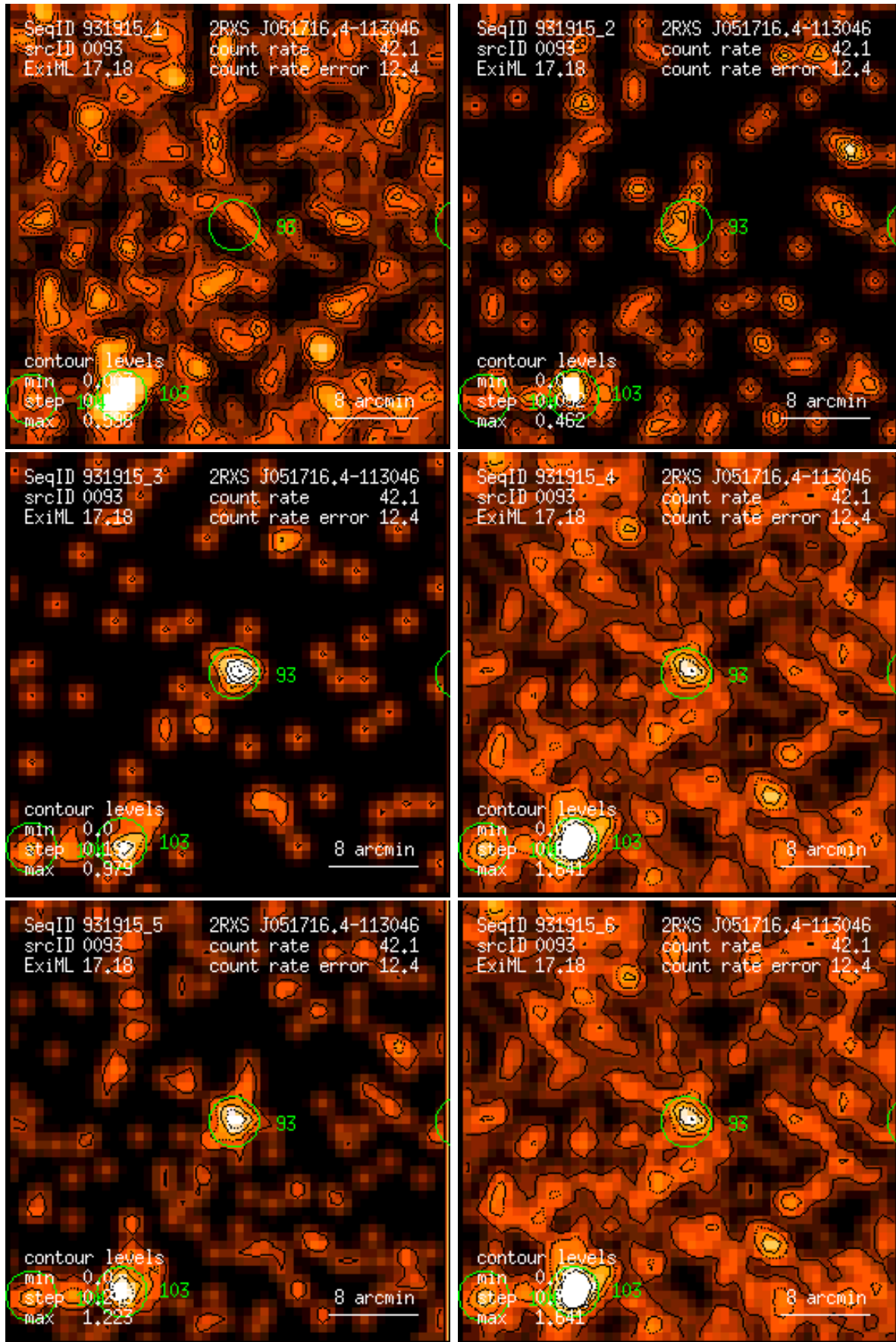
Figure 93: RASS 931915: detection 0093: band rate images, Gaussian filter: (1) PSPC channels 11 – 41, (2) 52 – 90, (3) 91 – 201, (4) 11 – 235, (5) 52 – 201, (6) 11 – 201. Broad band rates in counts/ks. Band rate contour levels in counts/ks/arcmin 2 .
