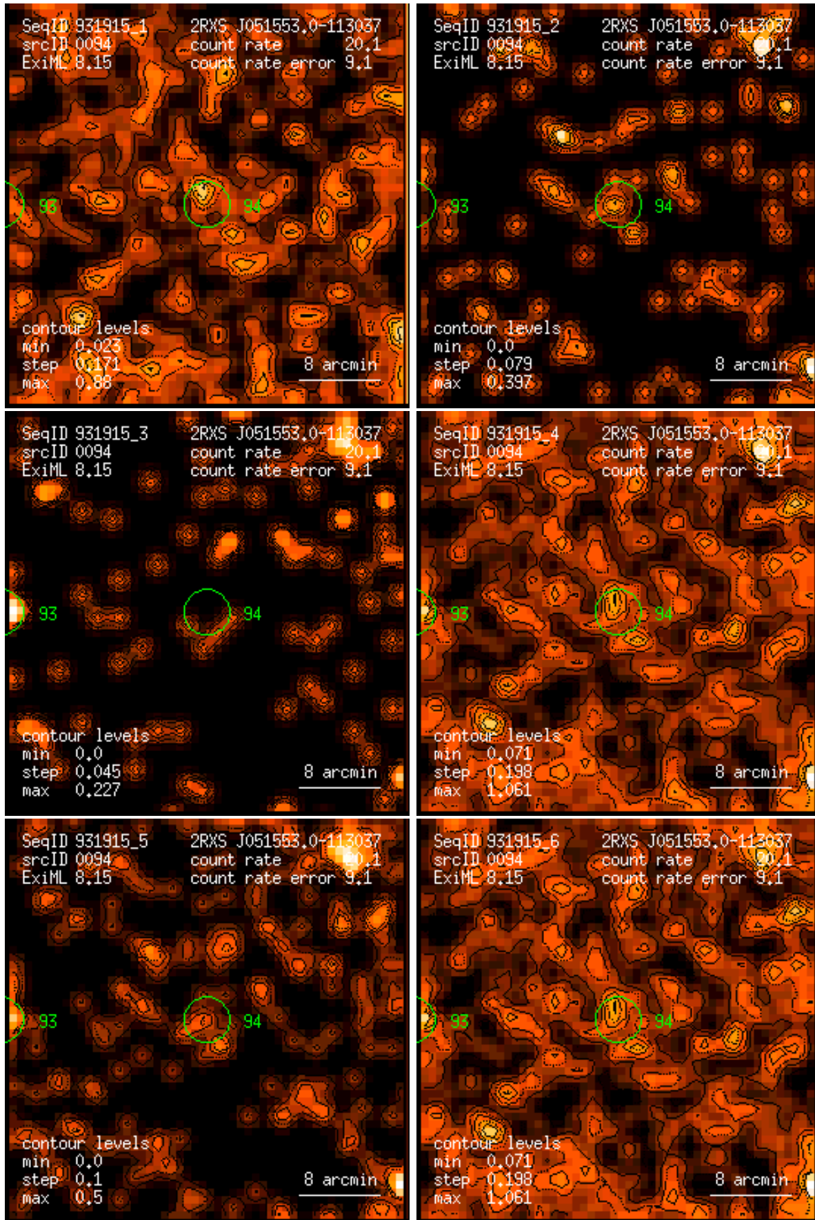
Figure 94: RASS 931915: detection 0094: band rate images, Gaussian filter: (1) PSPC channels 11 – 41, (2) 52 – 90, (3) 91 – 201, (4) 11 – 235, (5) 52 – 201, (6) 11 – 201. Broad band rates in counts/ks. Band rate contour levels in counts/ks/arcmin 2 .
