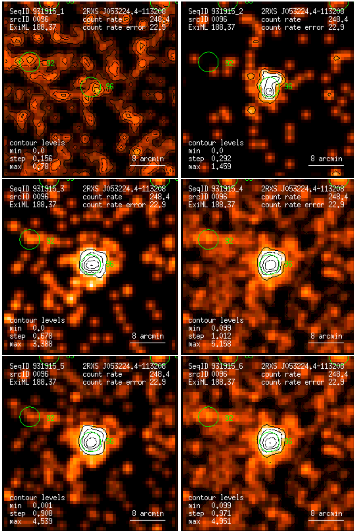
Figure 96: RASS 931915: detection 0096: band rate images, Gaussian filter: (1) PSPC channels 11 – 41, (2) 52 – 90, (3) 91 – 201, (4) 11 – 235, (5) 52 – 201, (6) 11 – 201. Broad band rates in counts/ks. Band rate contour levels in counts/ks/arcmin 2 .
