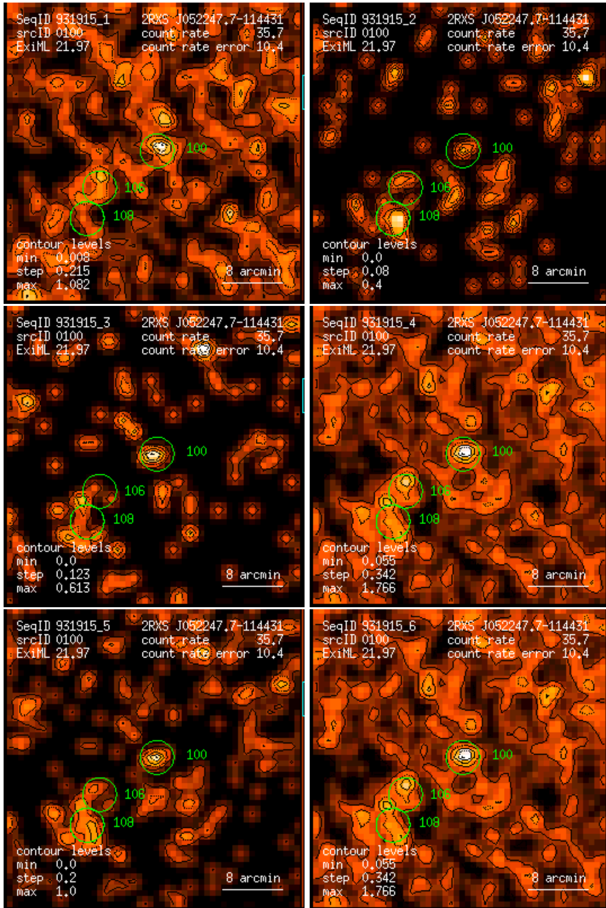
Figure 100: RASS 931915: detection 0100: band rate images, Gaussian filter: (1) PSPC channels 11 – 41, (2) 52 – 90, (3) 91 – 201, (4) 11 – 235, (5) 52 – 201, (6) 11 – 201. Broad band rates in counts/ks. Band rate contour levels in counts/ks/arcmin 2 .
