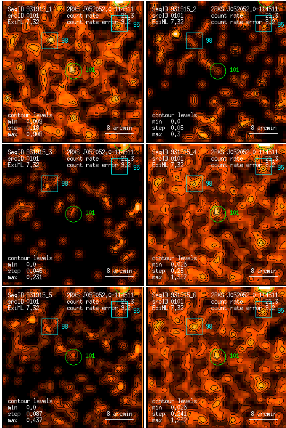
Figure 101: RASS 931915: detection 0101: band rate images, Gaussian filter: (1) PSPC channels 11 – 41, (2) 52 – 90, (3) 91 – 201, (4) 11 – 235, (5) 52 – 201, (6) 11 – 201. Broad band rates in counts/ks. Band rate contour levels in counts/ks/arcmin 2 .
